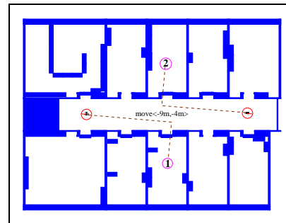
Fig. 3. Absolute positions of target points.
