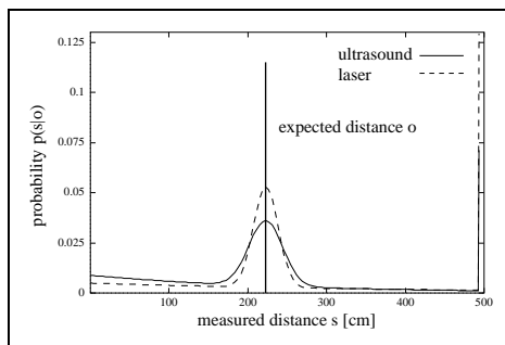
Fig. 1. Sensor model of ultrasound sensors and laser-range finders.
