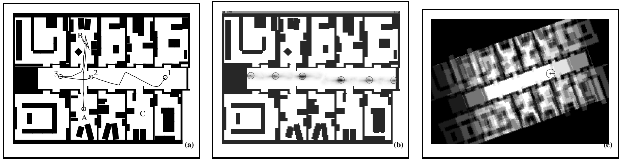
Fig. 4. (a) Environment and path of the robot. (b) Belief Bel(L) and (c) occupancy probabilities p_{occ}(a) at pos. 2.
