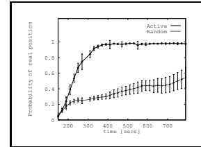
Fig. 10. Probability assigned to correct position.
