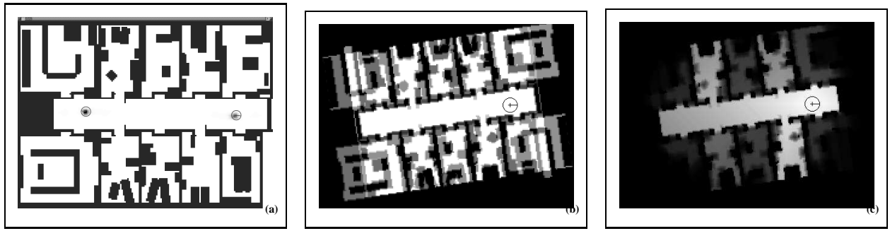
Fig. 6. (a) Belief Bel(L) at pos. 3, (b) occupancy probabilities p_{occ}(a) , and (c) expected costs C(a) .
