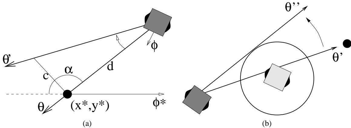
Figure 2: (a) The adjustment of \theta to \theta' to reach a target configuration of the form (x^*, y^*, \phi^*) ; (b) The adjustment of \theta' to \theta'' to avoid immediate obstacles.
