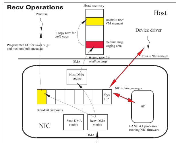
Figure 2: Data paths for sending and receiving short, medium, and bulk active messages. Short messages are transferred using programmed I/O directly on endpoints in NIC memory. Medium messages are sent and received using per-endpoint medium message staging areas in the pageable kernel heap that are mapped into a process's address space. A medium message is a single-copy operation at the sending host and a zero-copy operation at the receiving host. Bulk memory transfers, currently built using medium messages, are single-copy operations on the sender and single-copy operations on the receiver.
