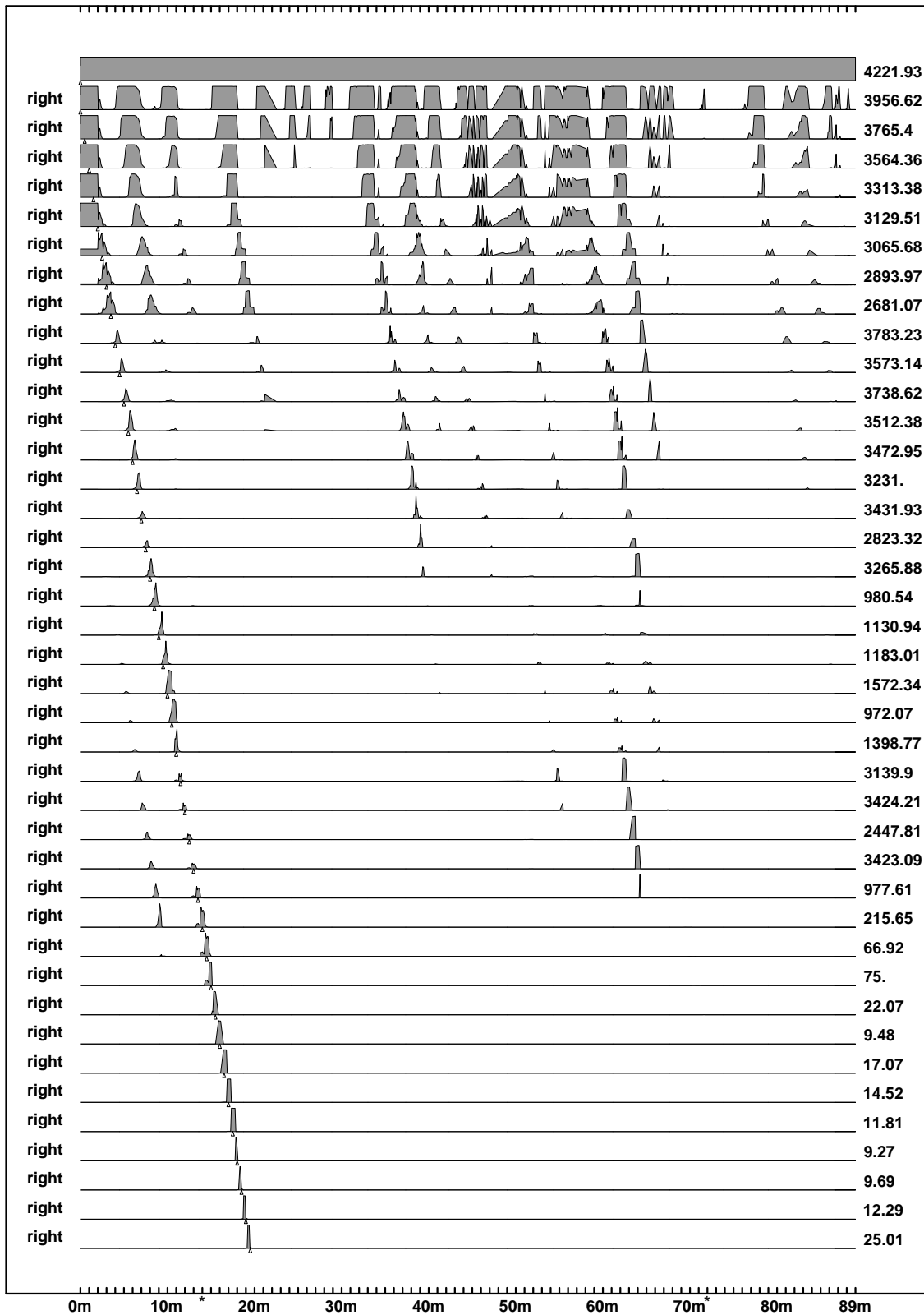
Figure 19: Localization with passive perception: Looking right.
