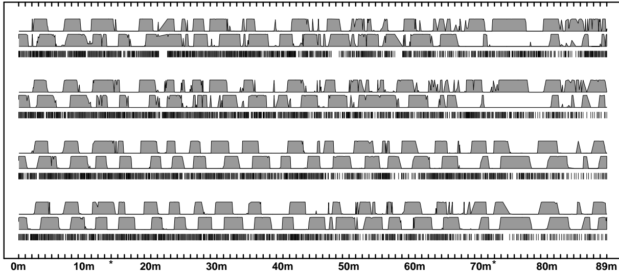
Figure 12: Landmarks selected by the robot with n = 2 networks.
