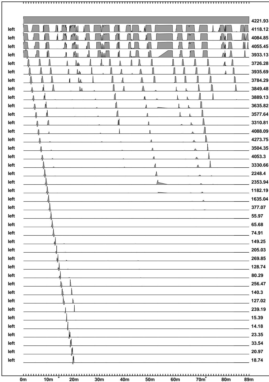
Figure 17: Localization with passive perception: Looking left.
