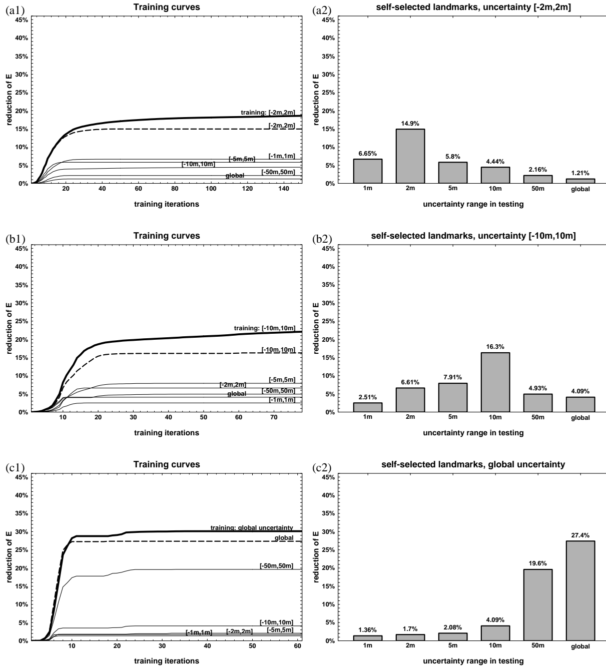
Figure 10: Results for self-selected landmarks.
