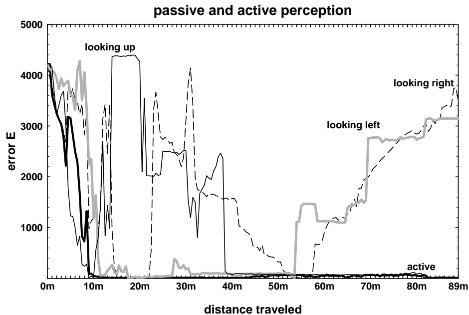
Figure 20: Localization error for passive and active perception. Notice that the error for active perception (thick solid line) stays close to zero after approx. 9 meters of robot motion.
