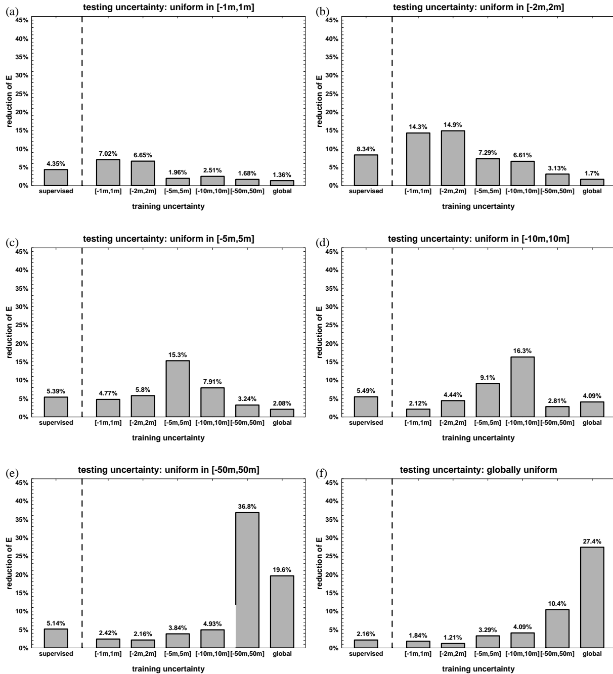
Figure 11: Performance comparison: supervised learning and self-selected landmarks, for different training and testing uncertainties.
