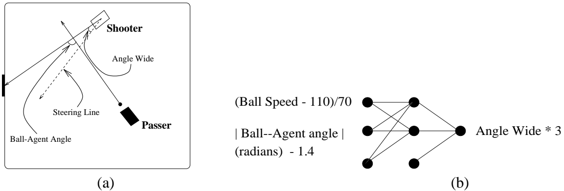
Figure 7: (a) The predicates we used to describe the world for the purpose of learning an aiming policy. (b) The neural network used to learn the aiming policy. The neural network has 2 hidden units with a bias unit at both the input and hidden layers.
