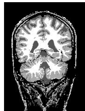
Gaussian labeling of corrected B20-PD/T2 Figure 17
