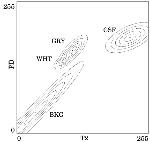
Isoprobability curves of approximated PD-versus- T2 distribution of the testing data (A25) Figure 6
