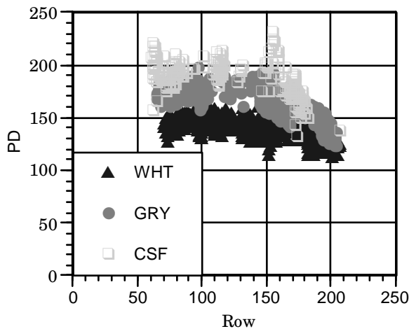
PD-versus-Row scattergram of the testing data (A25) Figure 5
