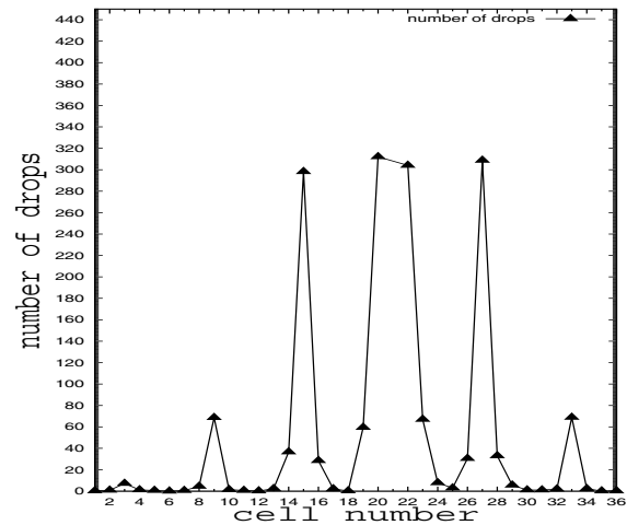
Fig. 12. Preferential mobility based hotspot: The number of drops vs. the cell number in a network scenario with 100% probability of going to a hotspot. Drops occurring in the cells are not uniform; cells closer to the hotspot cells have more drops than cells further away.
