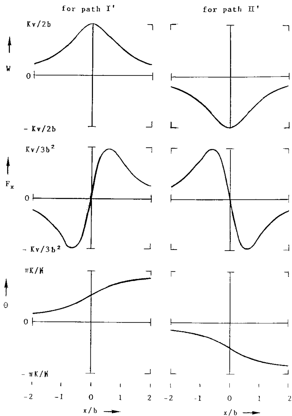
Figure 2. Weber potential W , the force of motional induction F_x , and the phase change \Theta as functions of the position x of an electron passing below the solenoid along path I' and above the solenoid along path II'.
