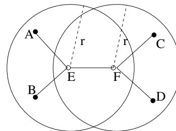
Fig. 9. Iterative MDS
