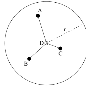
Fig. 8. Classical MDS
