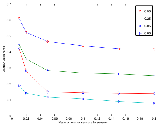
Fig. 13. Errors when applying the distributed positioning method with anchor sensors to all sensors in a square region with a uniform radio range and different distance measurement errors
