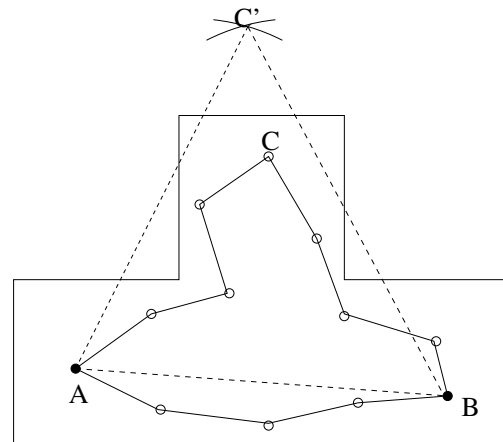
Fig. 2. Sensor Network in non-square area
