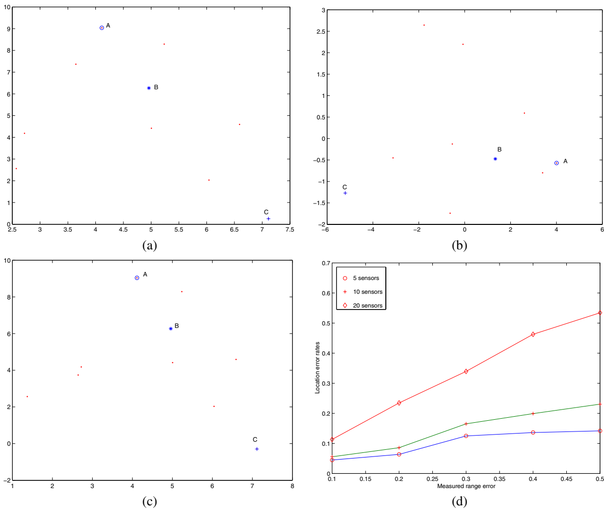
Fig. 11. (a)The physical positions of sensors in a adjacent area.(b) The recovered relative positions of sensors in the adjacent area based on classical MDS. (c) These sensors' physical positions after alignment. (d)When the error of measured distances for pairwise adjacent sensors increases, the error rates of estimated sensor positions increases.
