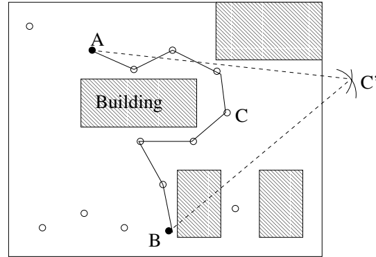
Fig. 1. Sensor Network deployed in a square area with obstacles
