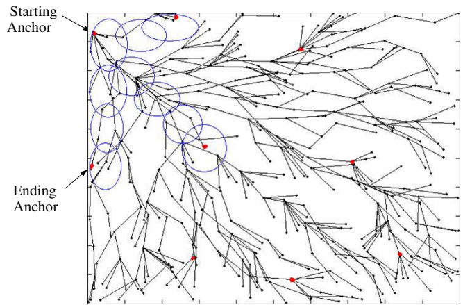
Fig. 5. Flooding from a starting anchor to the whole network. Red nodes are anchor nodes.
