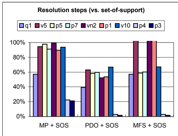
Figure 5: Performance comparison of three combinations of reasoning strategies. In contrast to Figure 2, the vertical axis is normalized relative to SOS.
