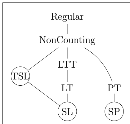
Figure 3: Subregular classes of sets with proper inclusion relationships indicated from top to bottom. TSL =Tier-based Strictly Local. LTT =Locally Threshold Testable. LT =Locally Testable. SL =Strictly Local. PT =Piecewise Testable. SP =Strictly Piecewise. Circled names indicate regions hypothesized to be where all individual phonotactic generalizations lie.
