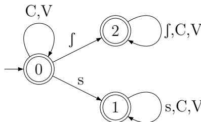
Figure 2: A finite-state acceptor recognizing the sibilant harmony pattern of Navajo. Symbol [s] stands for any anterior strident; [f] stands for any nonanterior strident; C stands for any nonstrident consonant; and V stands for any vowel.
