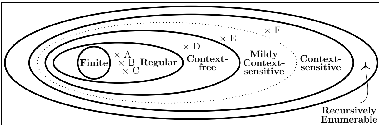
Figure 1: The Chomsky Hierarchy. Point A represents English consonant cluster constraints (Clements and Keyser, 1983); B is sibilant harmony in Samala Chumash (Applegate, 1972); C is the unbounded stress pattern of Kwakiutl (Bach, 1975); D is English nested embedding (Chomsky, 1956); E is a dialect of Swiss German (Shieber, 1985); and F is copying constructions in Yoruba relative clauses (Kobele, 2006).
