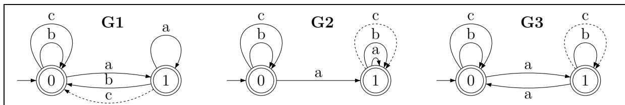
Figure 4: Finite-state grammars for three regular patterns. G1 maintains a short term memory w.r.t. [a] (i.e. State 1 means “just observed [a]”). G2 maintains a long-term memory w.r.t. [a] (i.e. State 1 means “observed [a] (sometime)”). G3 maintains a memory of the even/odd parity of [a]s (i.e. State 1 means “observed an even number of [a]s”). If dashed transitions are omitted, then G1 generates/recognizes all words except those with a forbidden string [ac]; G2 generates/recognizes all words except those with a forbidden subsequence [a...c]; and G3 generates/recognizes all words except those with a [c] whose left context contains an even number of [a]s. G1 is Strictly 2-Local, G2 is Strictly 2-Piecewise, and G3 is Counting.
