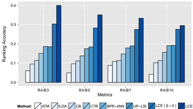
Figure 2: Comparison of the different methods on the Yahoo! News dataset.
