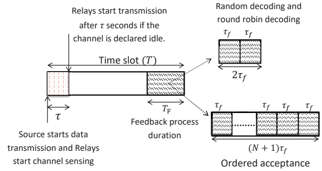
Fig. 1. Time slot structure under the proposed decoding strategies.
