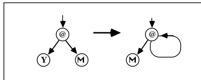
Figure 1. Cyclic Y-rule.
