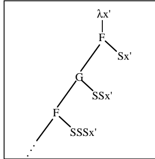
Figure 40. Partial tree.
