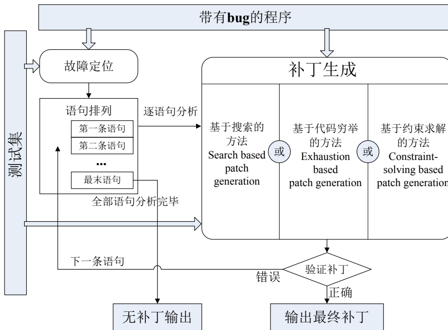
Fig.1 Overview of test-suite based repair 图 1 基于测试集的程序修复方法的流程概览
