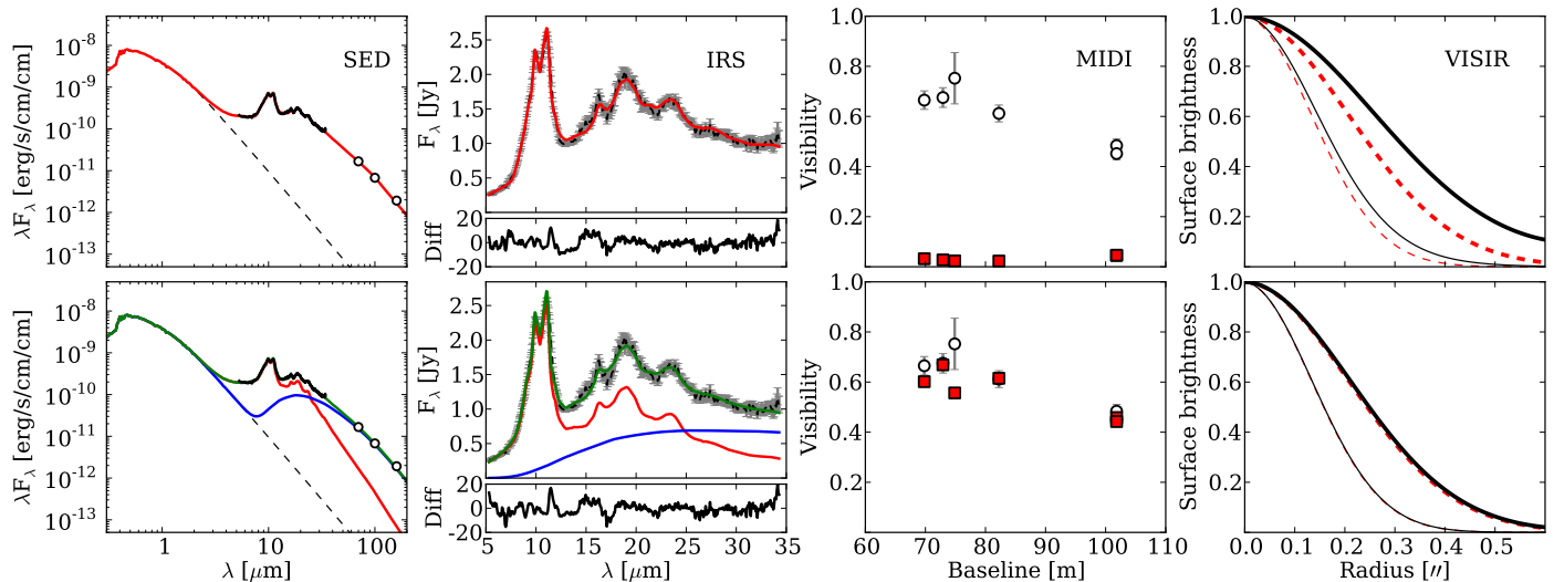
Fig. 3. Upper and lower panels: Results for the “1B” and “2B” models. Left panel: SED of HD 113766 A. The Irs spectrum is in black, Pacs data are shown as black open circles. For the “1B” model, the final best fit is in red. For the “2B” model, the final total fit is in green, the separate contributions of the inner and outer belts are in red and blue, respectively. Middle left panel: blow-up of the stellar subtracted Irs spectrum. Color coding is the same as for the left panel. Residuals ( 100 \times [F_{\nu,\text{obs}} - F_{\nu,\text{mod}}]/F_{\nu,\text{obs}} ) are displayed below the spectra. Middle right panel: Observed and modelled MIDI visibilities as a function of the baseline (open black circles and red squares, respectively, with 1\sigma uncertainties). Right panel: modelled surface brightness at 10 and 20\mu\text{m} (thin and thick black lines, respectively) of synthetic images convolved with 2D Gaussian with FWHM of 0.322'' and 0.498'' . The 2D Gaussian with the aforementioned FWHM, assumed to be PSF representative of the images, are shown in thin and thick dashed red lines, for comparison.
