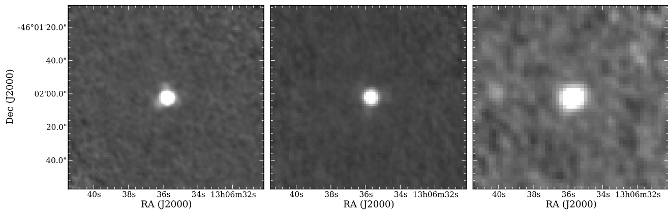
Fig. 1. Herschel/PACS observations at 70, 100, and 160 \mu\text{m} (left to right, respectively).
