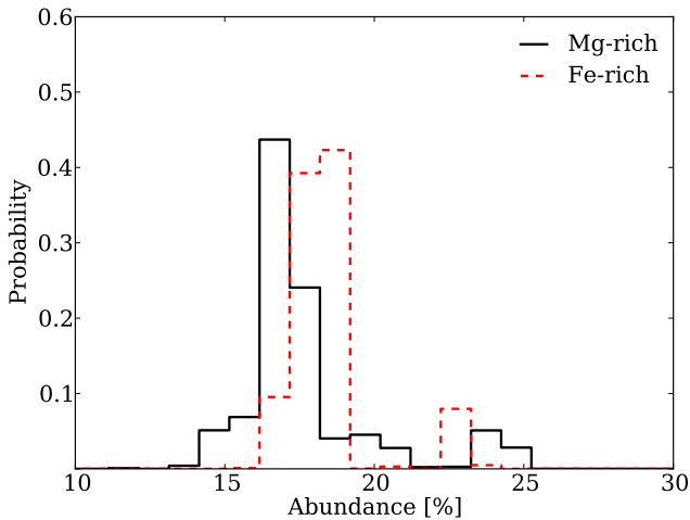
Fig. 4. Probability distributions from the MCMC run for model “2B”, as a function of relative abundances of Mg- and Fe-rich olivine grains (solid black, and dashed red, respectively).
