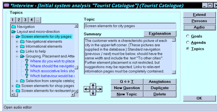
Figure 1. Main window of the interview assistant in RASSI
