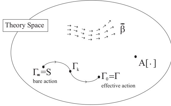
Fig. 1 The points of theory space are the action functionals A[\cdot] . The RG equation defines a vector field \vec{\beta} on this space; its integral curves are the RG trajectories k \mapsto \Gamma_k . They emanate from the fixed point action \Gamma_* \equiv \Gamma_\infty , which might differ from the bare action by a simple explicitly known functional, and end at the standard effective action \Gamma .
