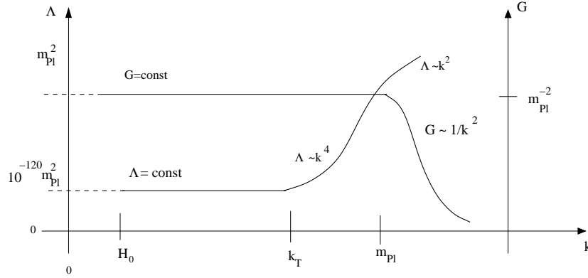
Fig. 3 The dimensionful \Lambda(k) \equiv \bar{\lambda}(k) and G(k) for a Type IIIa trajectory with realistic parameters.
