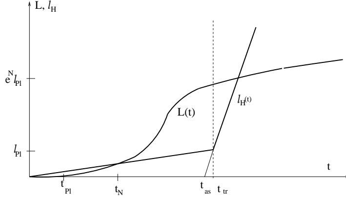
Fig. 8 Shown is the proper length L and the Hubble radius as a function of time. The NGFP and FRW cosmologies are valid for t < t_{\text{tr}} and t > t_{\text{tr}} , respectively. The classical cosmology has an apparent initial singularity at t_{\text{as}} outside its domain of validity. Structures of size e^N \ell_{\text{Pl}} at t_{\text{tr}} cross the Hubble radius at t_N , a time which can be larger than the Planck time.
