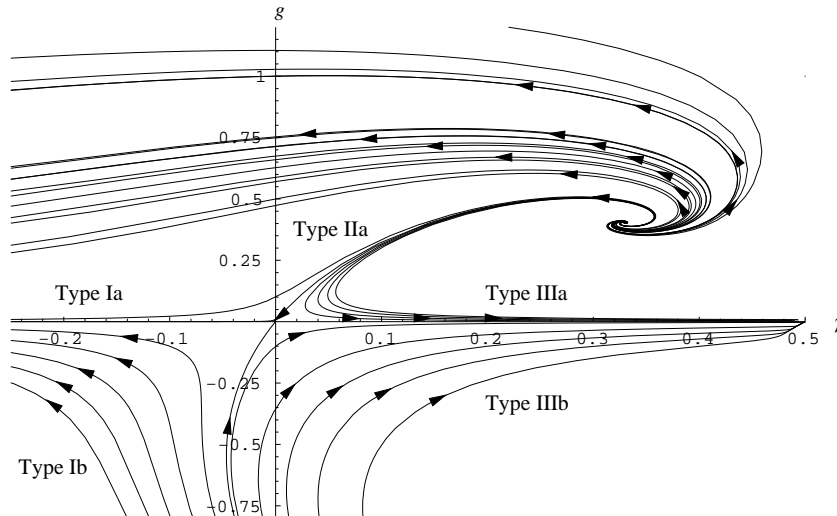
Fig. 2 RG flow in the g - \lambda -plane. The arrows point in the direction of increasing coarse graining, i.e., of decreasing k . (From [11].)
