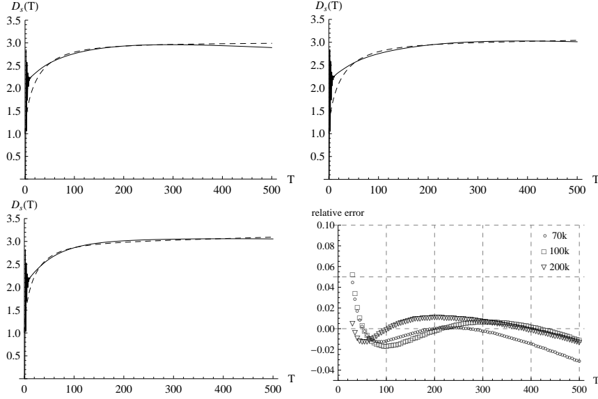
Fig. 6 Comparison between the spectral dimension measured in 3-dimensional CDT space-times build from 70k (upper left), 100k (upper right), and 200k simplices (lower left) obtained in [63] (continuous curves) and the best fit values for \mathcal{D}_s^{\text{QEG}}(T; g_0^{\text{fit}}, \lambda_0^{\text{fit}}) (dashed curves). The relative errors for the fits to the CDT-datasets with N = 70.000 (circles), N = 100.000 (squares) and N = 200.000 (triangles) simplices are shown in the lower right. The residuals grow for very small and very large durations T of the random walk, consistent with discreteness effects at small distances and the compactness of the simulation for large values of T , respectively. The quality of the fit improves systematically for triangulations containing more simplices. For the N = 200k data the relative error is \approx 1\% .
