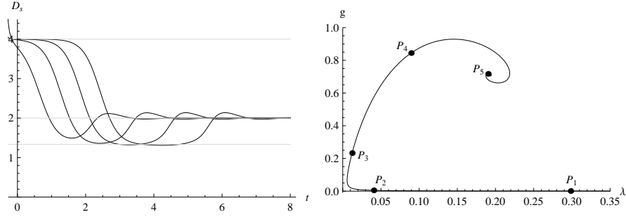
Fig. 5 The t \equiv \ln(k) -dependent spectral dimension along illustrative solutions of the RG-equations (18) in d = 4 . The trajectories develop three plateaus: the classical plateau with \mathcal{D}_s = 4, \mathcal{D}_w = 2 , the semi-classical plateau where \mathcal{D}_s = 4/3, \mathcal{D}_w = 6 and the NGFP plateau with \mathcal{D}_s = 2, \mathcal{D}_w = 4 . (Recall that \mathcal{D}_w = 2d/\mathcal{D}_s = 8/\mathcal{D}_s .) The plateau values are indicated by the horizontal lines. The second figure shows the location of these plateaus on the RG trajectory: the classical, k^4 , and NGFP regime appear between the points P_1 and P_2, P_3 and P_4 , and above P_5 , respectively.
