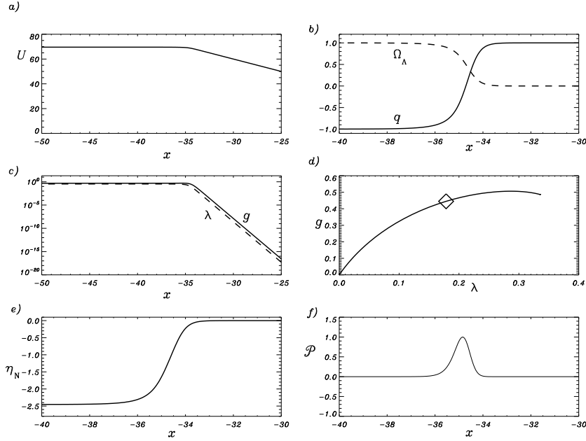
Fig. 9 The crossover epoch of the cosmology for \Omega_\lambda^* = 0.98 . The plots a) , b) , c) display the logarithmic Hubble parameter \mathcal{U} , as well as q , \Omega_\lambda , g and \lambda as a function of the logarithmic scale factor x . A crossover is observed near x \approx -34.5 . The diamond in plot d) indicates the point on the RG trajectory corresponding to this x -value. (The lower horizontal part of the trajectory is not visible on this scale.) The plots e) and f) show the x -dependence of the anomalous dimension and entropy production rate, respectively.
