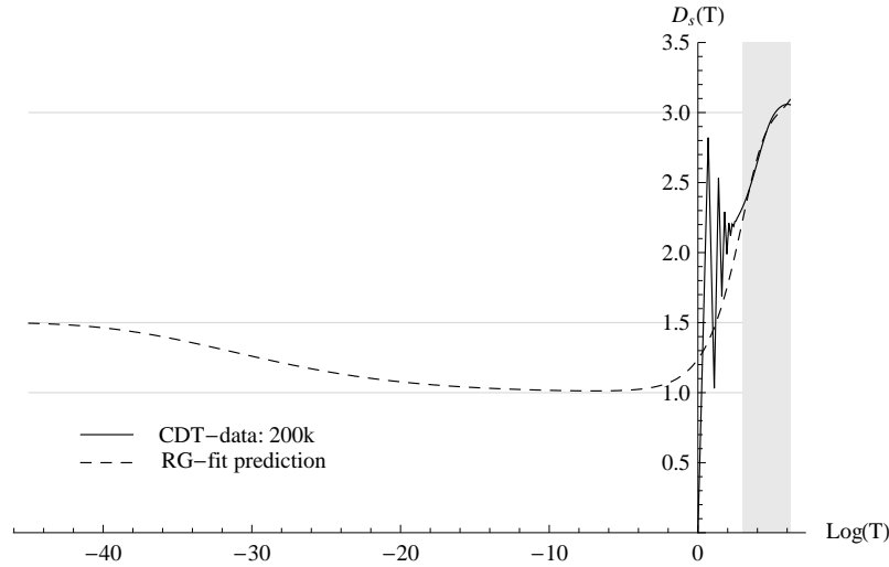
Fig. 7 Comparison between the spectral dimensions obtained from the dynamical triangulation with 200k simplices (continuous curve) and the corresponding \mathcal{D}_s^{\text{QEG}}(T; g_0^{\text{fit}}, \lambda_0^{\text{fit}}) predicted by QEG (dashed curve). In the latter case, the scaling regime corresponding to the NGFP is reached for \log(T) < -40 , which is well below the distance scales probed by the Monte Carlo simulation.
