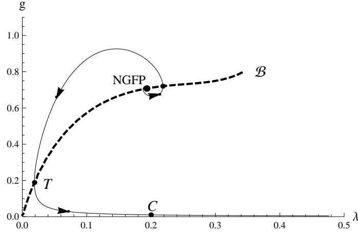
Fig. 4 The g - \lambda -theory space with the line of turning points, \mathcal{B} , and a typical trajectory of Type IIIa. The arrows point in the direction of decreasing k . The big black dot indicates the NGFP while the smaller dots represent points at which the RG trajectory switches from increasing to decreasing \lambda or vice versa. The point T is the lowest turning point, and C is a typical point within the classical regime. For \lambda \gtrsim 0.4 , the RG flow leaves the classical regime and is no longer reliably captured by the Einstein-Hilbert truncation.
