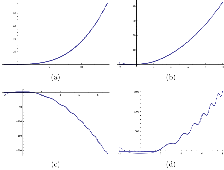
Figure 2: (a) The perturbative, (b) 1-instanton, (c) 2-instanton and (d) 3-instanton corrections of the grand potential J_k(\mu) at k = 2 . The dots represent the grand potential obtained by the exact partition function while the solid lines represent the fitted functions.
