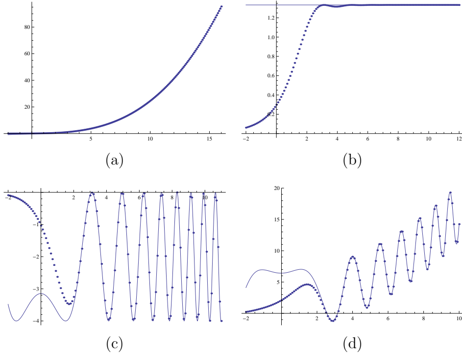
Figure 3: (a) The perturbative, (b) 1-instanton, (c) 2-instanton and (d) 3-instanton corrections of the grand potential J_k(\mu) at k = 3 . The dots represent the grand potential obtained by the exact partition function while the solid lines represent the fitted functions.
