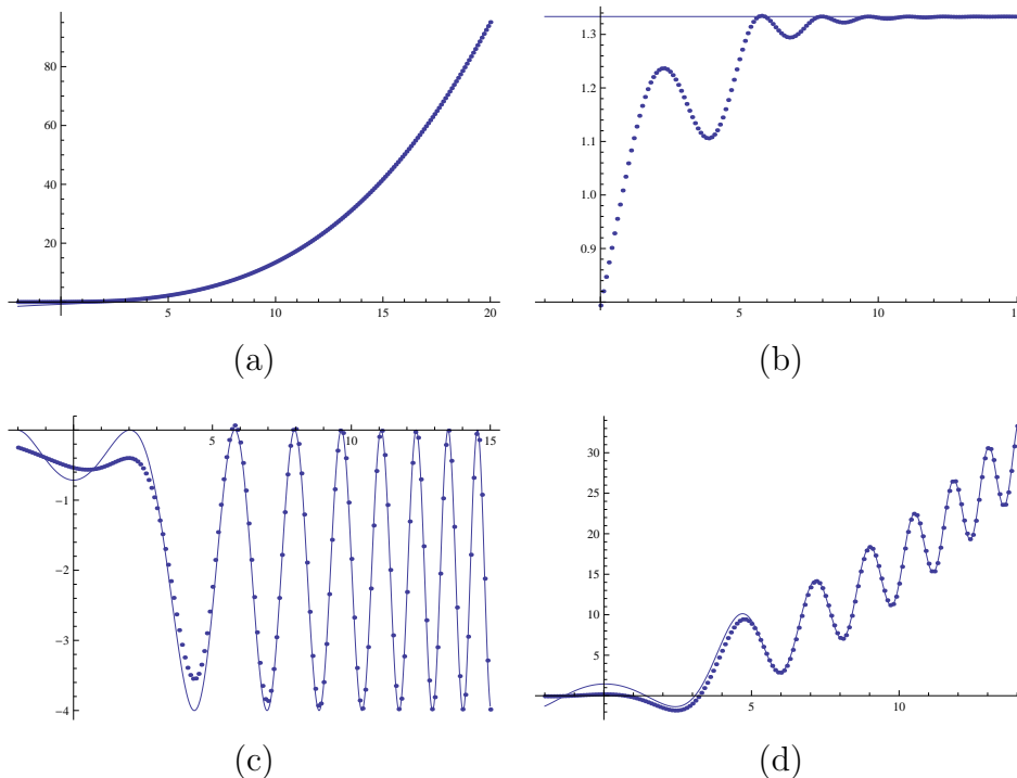
Figure 5: (a) The perturbative, (b) 1-instanton, (c) 2-instanton and (d) 3-instanton corrections of the grand potential J_k(\mu) at k = 6 . The dots represent the grand potential obtained by the exact partition function while the solid lines represent the fitted functions.
