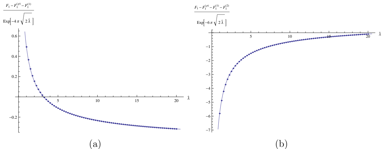
Figure 7: (a) The 2- and (b) 3-instanton corrections to the genus one free energy.
