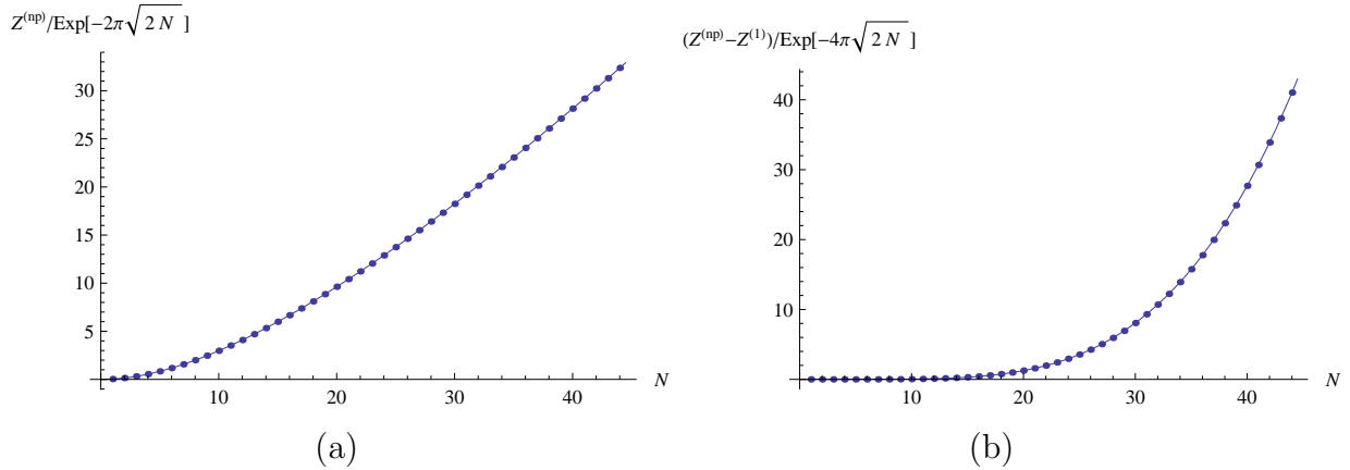
Figure 6: The 1- and 2-instanton corrections to the partition function at k = 1 . We plot (a) Z_1^{(\text{np})}/e^{-2\pi\sqrt{2N}} and (b) (Z_1^{(\text{np})} - Z_1^{(1)})/e^{-4\pi\sqrt{2N}} against N . The instanton corrections in terms of the Airy function (the solid lines) excellently agree with the exact values (the dots) even for small N .
