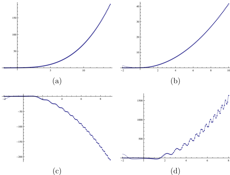
Figure 1: (a) The perturbative, (b) 1-instanton, (c) 2-instanton and (d) 3-instanton corrections of the grand potential J_k(\mu) at k = 1 . The dots represent the grand potential obtained by the exact partition function while the solid lines represent the fitted functions.
