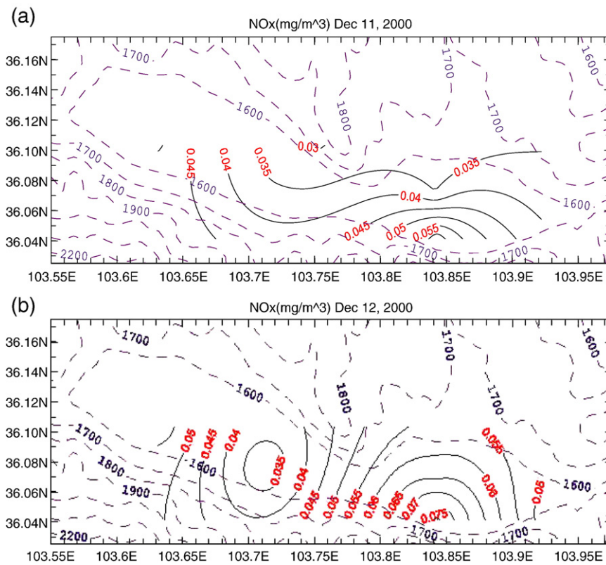
Fig. 10. Observed NO x concentration on (a) December 11, and (b) December 12, 2000.
