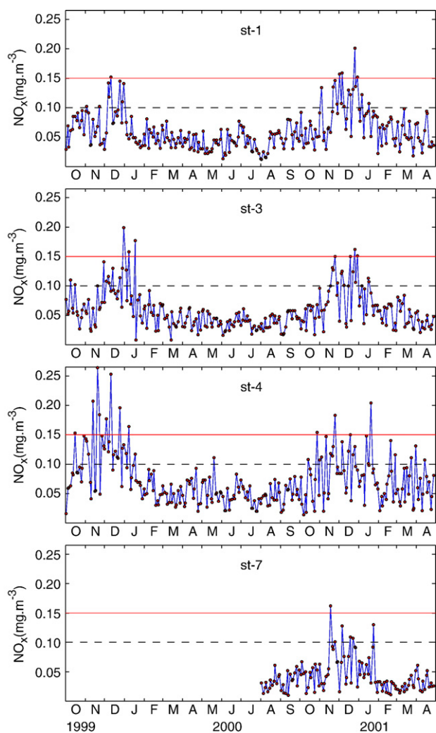
Fig. 4. Daily mean NO x concentrations (mg m -3 ) at St-1, St-3, St-4 and St-7 representing four districts. Horizontal dashed line is daily mean second-level criterion, while horizontal solid line is daily mean third-level criterion.
