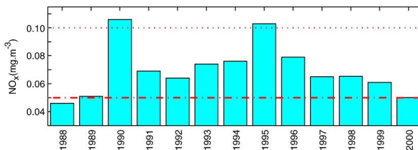
Fig. 3. Annual mean \text{NO}_x concentration ( \text{mg m}^{-3} ) measured at the local CEPA station ( 103.631^\circ\text{E} , 36.103^\circ\text{N} ), which is marked as the solid circle in Fig. 1b. The second-level criterion is represented by the horizontal dash-dotted line and the third-level criterion is represented by the horizontal dotted line.
