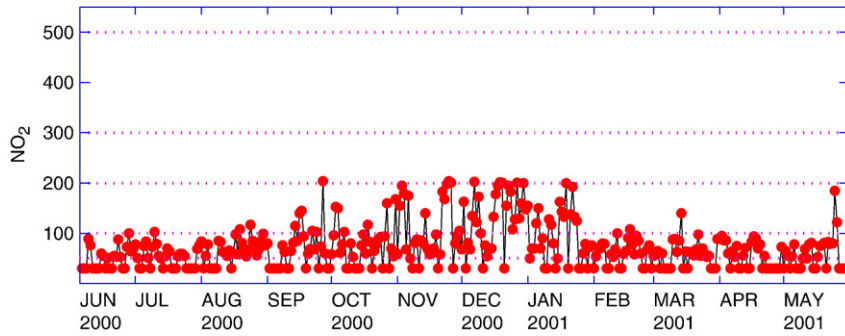
Fig. 5. Daily mean API of NO 2 at station-E.
