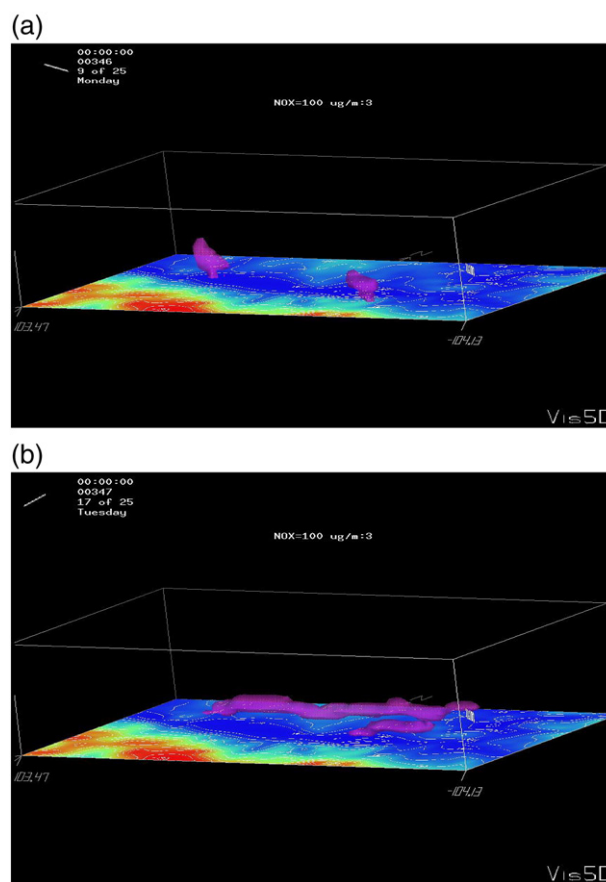
Fig. 9. Model simulated NO x plume (concentration >0.1 mg/m 3 ) spreading and enhancing from (a) 0700 BT, Dec 11 to (b) 0700 BT, Dec 12, 2000
