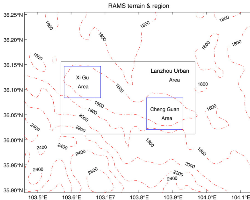
Fig. 11. Two areas of interest: (a) XiGu (industrial district), and (b) Cheng Guan (commercial and residential district).
