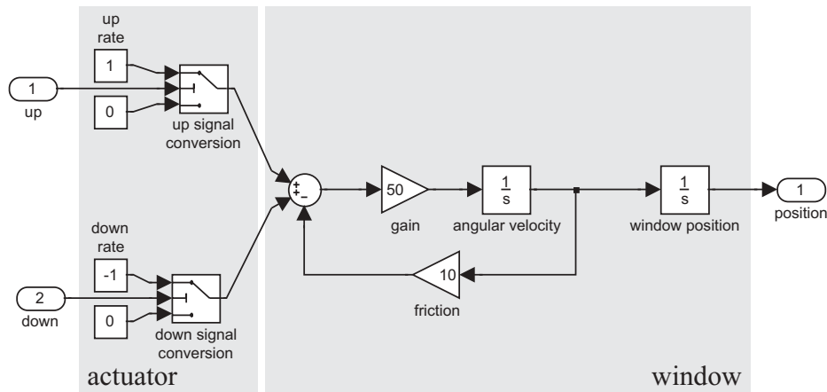
Figure 2. Low-order model of power window behavior
