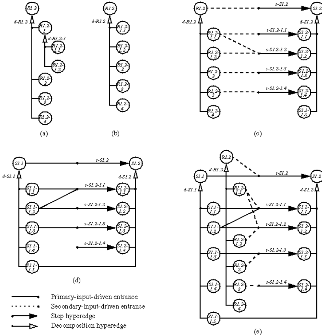
Figure 2: Relational hypergraphs
