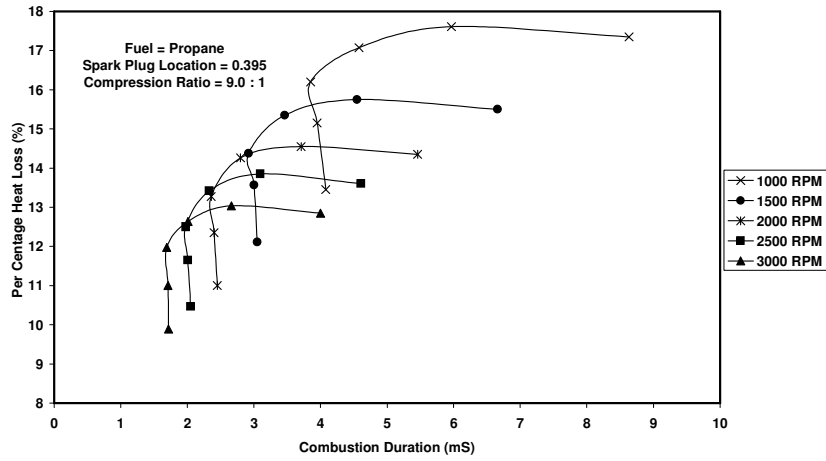
Figure 9. Variation of Per Cent Heat Loss with combustion duration at different engine speeds.
