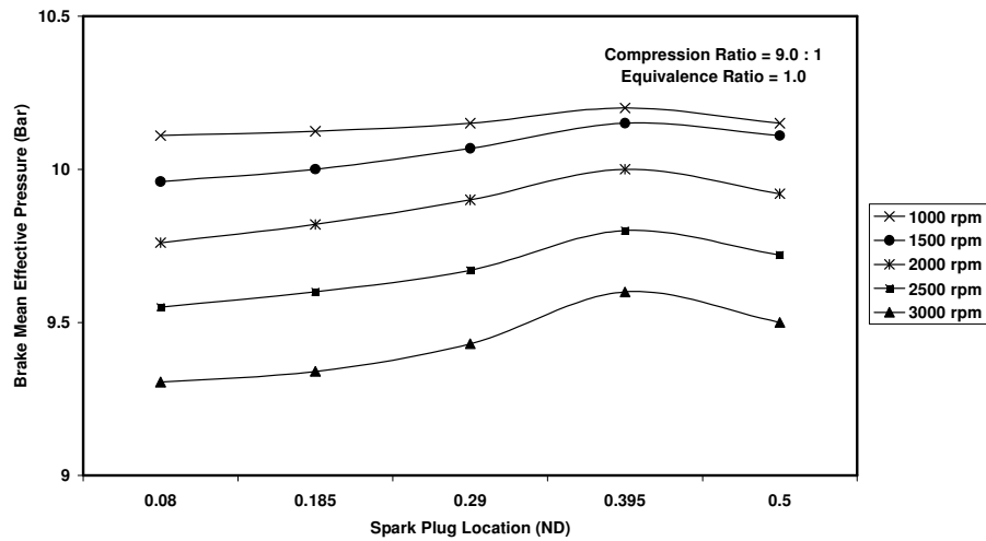
Figure 4-A. Variation of Brake Mean Effective Pressure with Spark Plug Location at different engine speeds.
