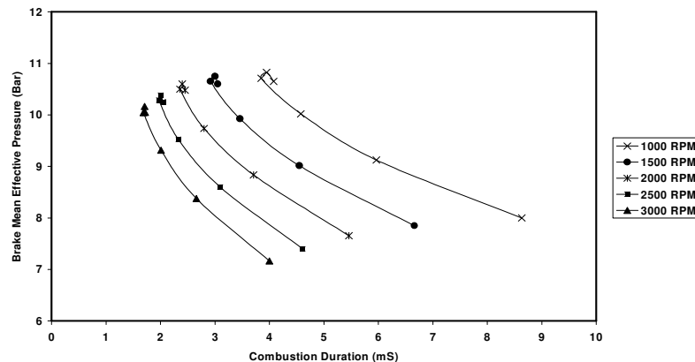
Figure 8. Variation of Brake Mean Effective Pressure with combustion duration at different engine speeds.
