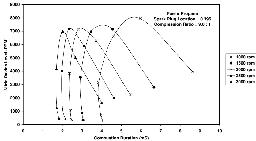
Figure 13. Variation of Nitric Oxide Level with combustion duration at different engine speeds.
