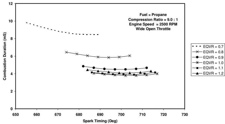
Figure 5. Variation of Combustion Duration with Spark Timing at different equivalence ratios.
