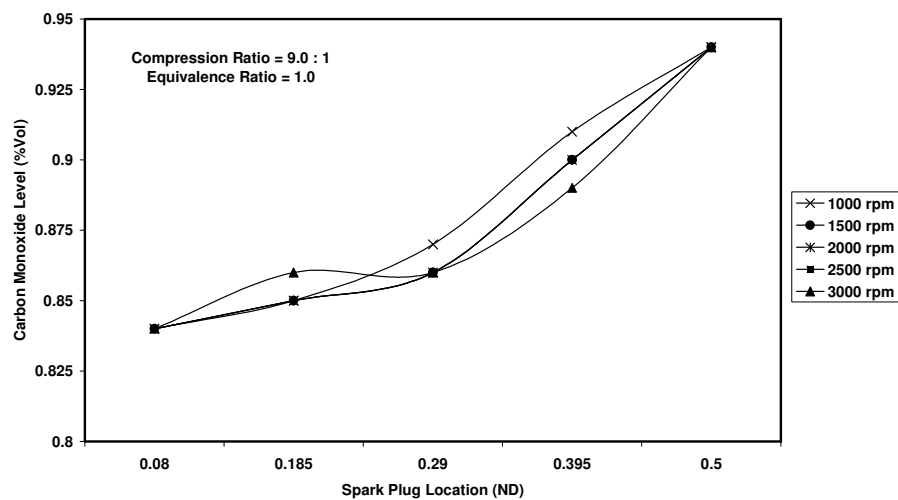
Figure 4-C. Variation of Carbon Monoxide Level with Spark Plug Location at different engine speeds.
