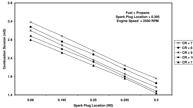
Figure 3. Variation of Combustion Duration with Spark Plug Location at different compression ratios
