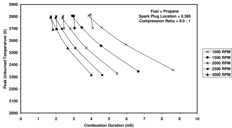
Figure 6. Variation of Peak Unburned Temperature with combustion duration at different engine speeds.
