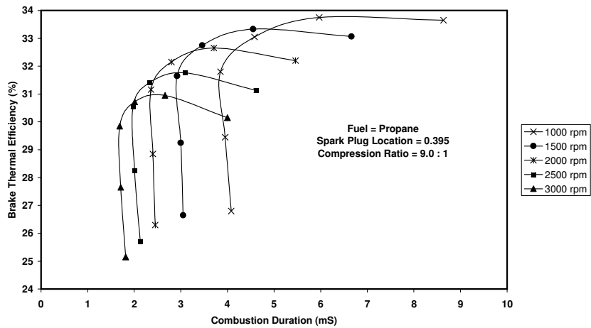
Figure 11. Variation of Brake Thermal Efficiency with combustion duration at different engine speeds.
