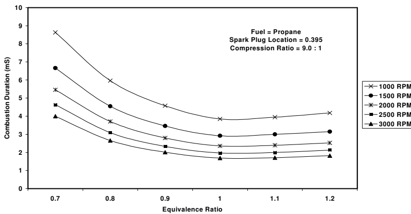
Figure 2. Variation of Combustion Duration with Equivalence Ratio at different engine speeds.
