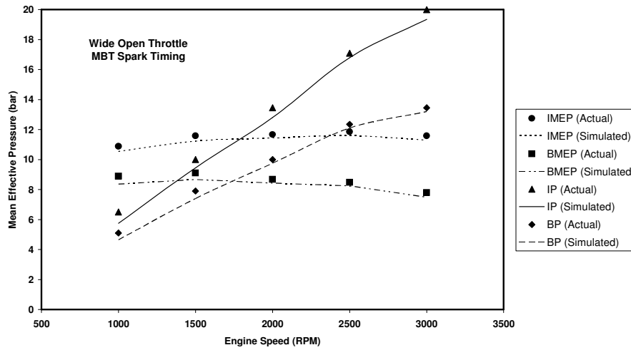
Figure 1-A. Performance Comparison between the experimental & theoretical results.
