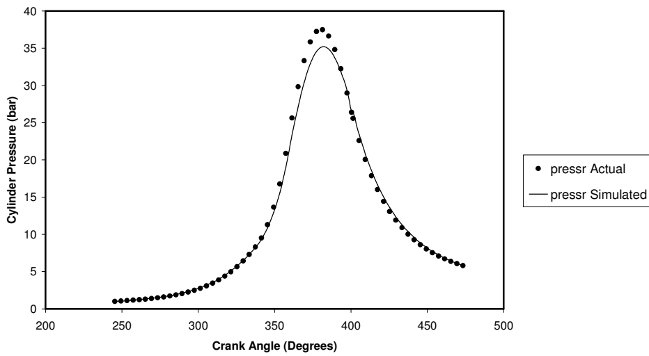
Figure 1-B. Pressure-Crank Angle comparison the experimental & theoretical results
