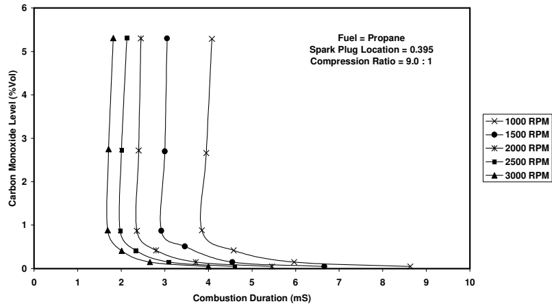
Figure 12. Variation of Carbon Monoxide Level with combustion duration at different engine speeds.
