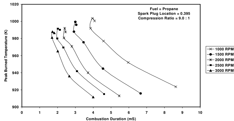
Figure 7. Variation of Peak Burned Temperature with combustion duration at different engine speeds.
