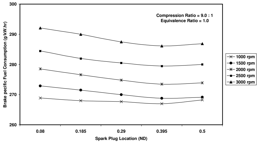
Figure 4-B. Variation of Brake Specific Fuel Consumption with Spark Plug Location at different engine speeds.
