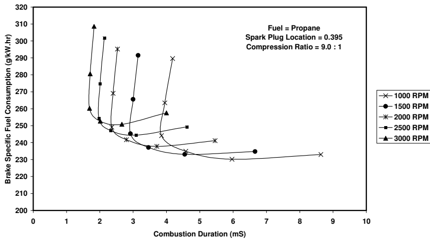
Figure 10. Variation of Brake Specific Fuel Consumption with combustion duration at different engine speeds.
