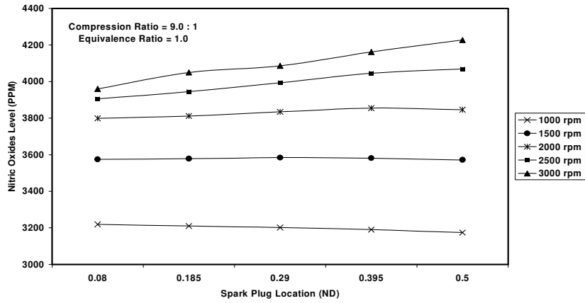
Figure 4-D. Variation of Nitric Oxide Level with Spark Plug Location at different engine speeds.
