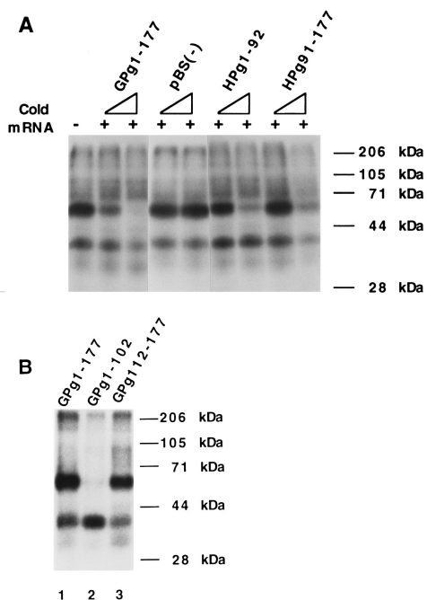
FIG. 7. p65 binds to the terminal region of GSHV pgRNA. (A) SDS-PAGE analysis of nuclear extract incubated with labeled GPg1-177 alone (lane 1) and in the presence of increasing amounts of unlabeled GPg1-177 (lanes 2 and 3), unlabeled RNA from pBS(-)T3 [pBS(-); lanes 4 and 5], and unlabeled HBV RNAs containing either UBS (HPg1-92; lanes 6 and 7) or DBS (HPg1-172; lanes 8 and 9). The molar excesses of unlabeled to labeled RNAs were 50-fold in lanes 2, 4, 6, and 8 and 250-fold in lanes 3, 5, 7, and 9. (B) SDS-PAGE analysis of nuclear extract incubated with labeled full-length GPg1-177 (lane 1), with labeled 5' half of the RNA (GPg1-102; lane 2), or with labeled 3' half of the RNA (GPg112-177; lane 3).
