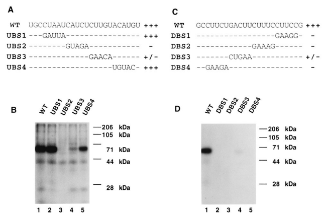
FIG. 5. Mutational analysis of p65 binding sites. (A) Sequence of the minimal region defining UBS and depiction of the nucleotide sequence changes introduced in each mutant RNA; at the right is a scoring of the binding assay as in Fig. 3B. WT, wild type. (B) SDS-PAGE analysis of nuclear extract UV cross-linked either to labeled HPg1-43 (lane 1) or to each of the indicated labeled mutant RNAs. (C) Sequence of the minimal region defining DBS and scheme of the changes made in each mutant RNA, with schematic scoring of the binding reaction at the right. (D) SDS-PAGE analysis of nuclear extract UV cross-linked either to labeled HPg141-172 (lane 1) or to each of the indicated labeled mutant RNAs.
