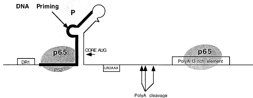
FIG. 8. Schematic depiction of landmarks within the 5' 172 nt of HBV pgRNA. The locations of p65 binding sites are noted with respect to elements known to influence various functions in which this region plays an important role in several hepadnaviruses (see the text for more details). Black bar, PS2 polyadenylation-enhancing element; DR1, extent of direct repeat sequence involved in DNA strand transfers; UAUAAA, HBV polyadenylation signal; arrows, poly(A) addition sites; long box, U-rich region required for accurate and efficient poly(A) addition.
