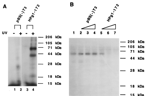
FIG. 1. Nuclear proteins bind to the 5' 172 nt of HBV pgRNA. (A) SDS-PAGE analysis of nuclear extract from HepG2 cells incubated with either labeled RNA from pBS(-) (lanes 1 and 2) or labeled HPg1-172 (lanes 3 and 4) and then either stored on ice (lanes 1 and 3) or UV cross-linked (lanes 2 and 4). (B) Competition experiment with unlabeled RNAs. The nuclear extract was incubated and UV cross-linked with labeled HPg1-172 only (lane 1) or with that RNA in the presence of increasing amounts of unlabeled RNA from pBS(-) (lanes 2 to 4) or HPg1-172 (lanes 5 to 7). The weight ratios of unlabeled to labeled RNA were 40-fold in lanes 2 and 5, 200-fold in lanes 3 and 6, and 280-fold in lanes 4 and 7.
