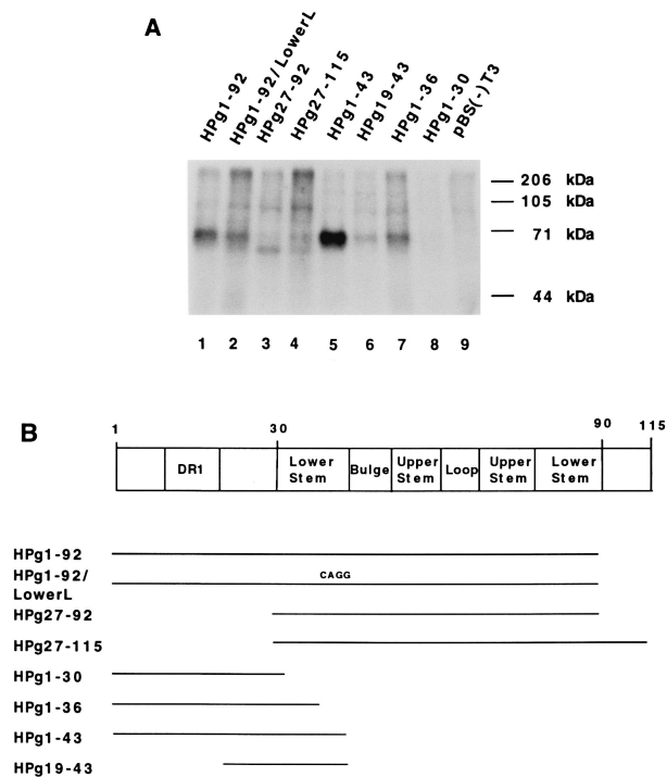
FIG. 3. Delimitation of UBS. (A) SDS-PAGE analysis of nuclear extract UV cross-linked to HPg1-92 (lane 1) and its derivatives containing deletions from the 5' end (lane 3), from the 3' end (lanes 5, 6, and 8), or from both ends (lane 6). In lane 2, the extract was UV cross-linked to HPg1-92 containing a mutation that destroyed the pairing in the lower stem of \epsilon , HPg1-92/LowerL (26). In lane 3, the labeled RNA, HPg27-115, contained a 5' deletion but included additional 3' sequence containing the poly(A) signal. (B) Scheme of the RNAs tested for their ability to be recognized by p65 with respect to the indicated sequence landmarks present in the first 92 nt of HBV pgRNA. At the right is shown a scoring of the UV cross-linking results: ++, 25 to 100% of wild-type binding; +, binding reduced to 10 to 25% of the wild-type level; -, less than 5 to 10% of wild-type binding.
