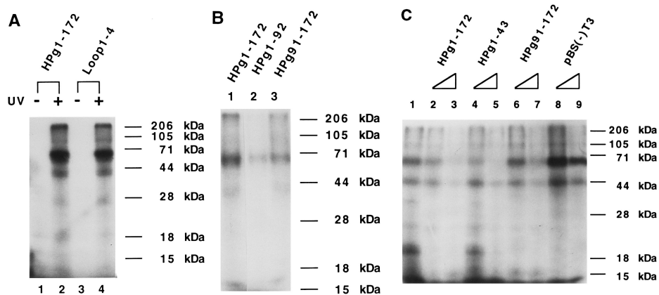
FIG. 2. p65 binds to two discrete binding sites. (A) SDS-PAGE analysis of nuclear extract incubated (all lanes) and UV cross-linked (lanes 2 and 4) with either labeled HPg1-172 (lanes 1 and 2) or labeled HPg1-172 containing loop mutation Loop1-4 (lanes 3 and 4). (B) SDS-PAGE analysis of nuclear extract incubated and UV cross-linked with labeled HPg1-172 (lane 1), labeled HPg1-92 (lane 2), or labeled HPg91-172 (lane 3). (C) Competition experiment with unlabeled RNAs. The nuclear extract was UV cross-linked to labeled HPg1-172 only (lane 1) or to this RNA in the presence of increasing amounts of unlabeled HPg1-172 (lanes 2 and 3), HPg1-43 (lanes 4 and 5), HPg91-173 (lanes 6 and 7), or RNA from pBS(-) (lanes 8 and 9). The molar excesses of unlabeled to labeled RNA were 50-fold in lanes 2, 4, 6, and 8 and 250-fold in lanes 3, 5, 7, and 9.
