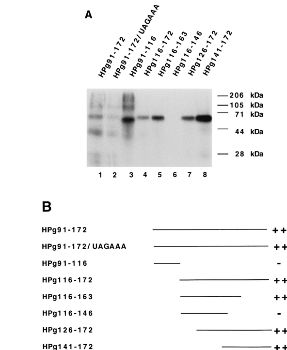
FIG. 4. Delimitation of DBS. (A) SDS-PAGE analysis of nuclear extract UV cross-linked to HPg91-172 (lane 1) and its derivatives containing deletions from the 5' end (lanes 4, 7, and 8), from the 3' end (lane 3), or from both ends (lanes 5 and 6). The RNA used in lane 2, HPg91-172, contained a mutated poly(A) site. (B) Scheme of the RNAs tested for the ability to be recognized by p65. At the right is a semiquantitative scoring of the binding results as in Fig. 3B.
