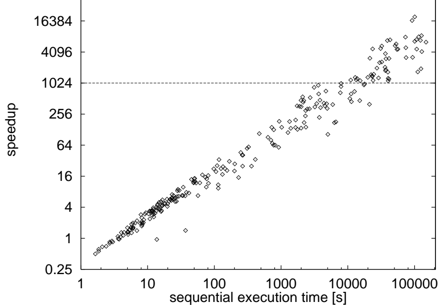
Figure 1: Speedup for 256 instances of the knapsack problem on 1024 PEs.
