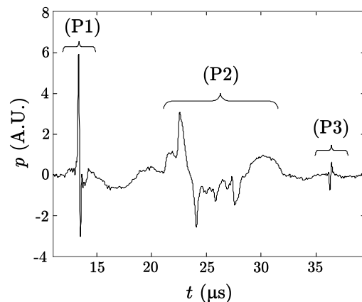
Fig. 2 Optoacoustic signal captured by the transducer, corresponding to the phantom experiment described in Fig. 1. The parts of the signals corresponding to different waves can be differentiated: directly propagating signal generated by the hair (P1), waves generated in the imaged object (P2), and the scattered hair signal (P3).
