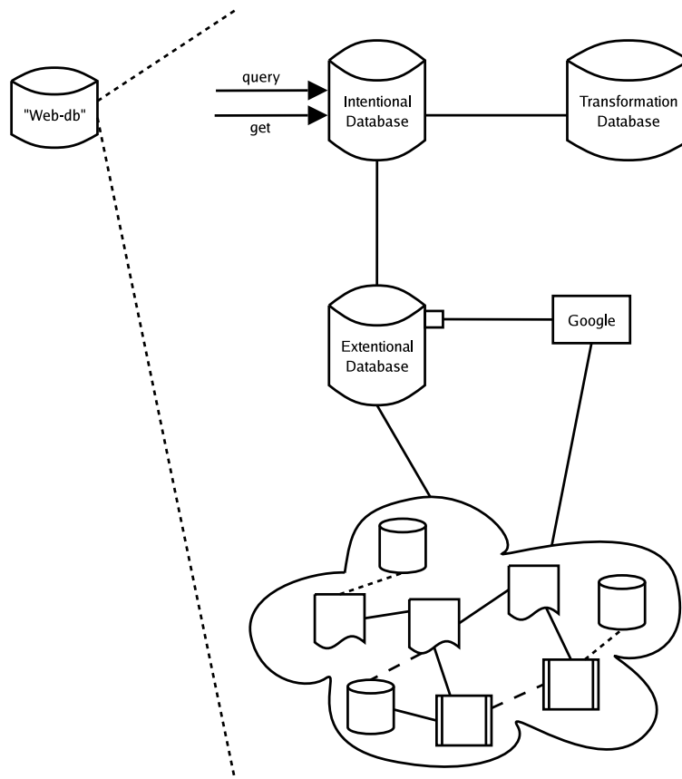
Figure 11. Implementation view on Vimes
