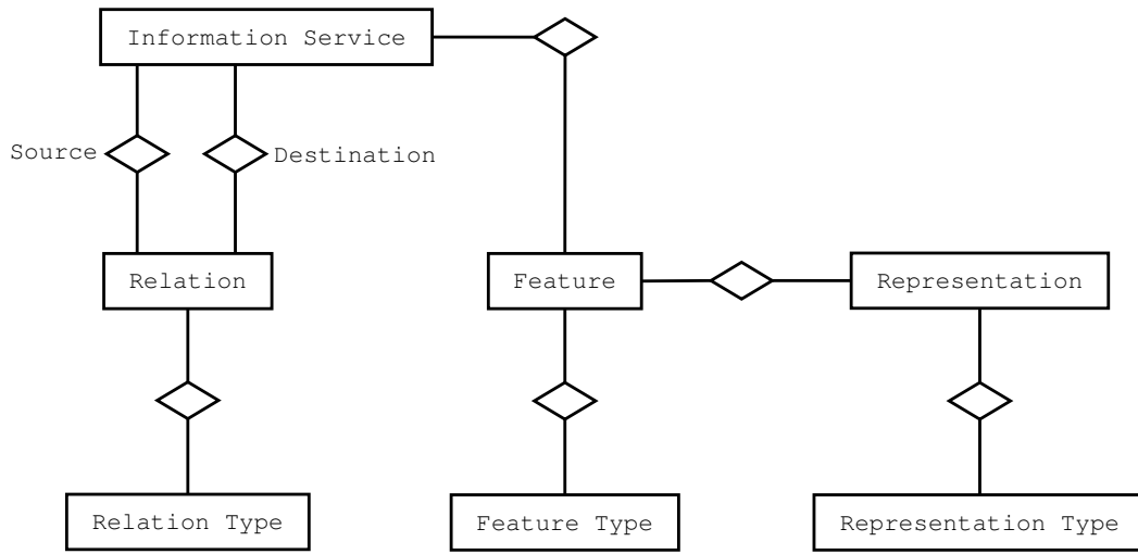
Figure 5. Typing of Features and Representations
