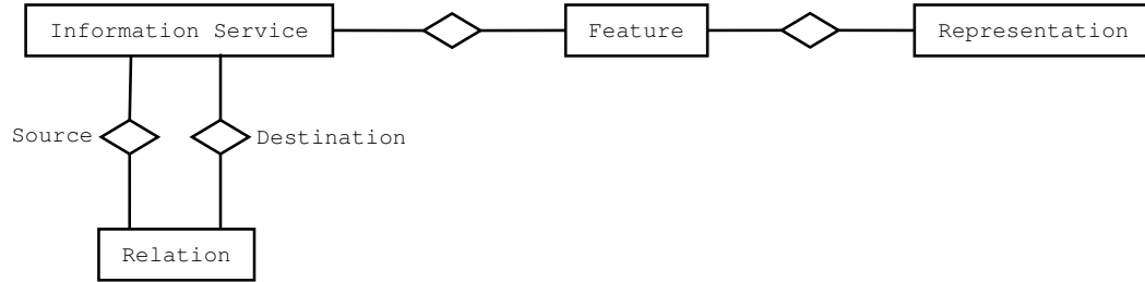
Figure 4. Information Services and Relations
