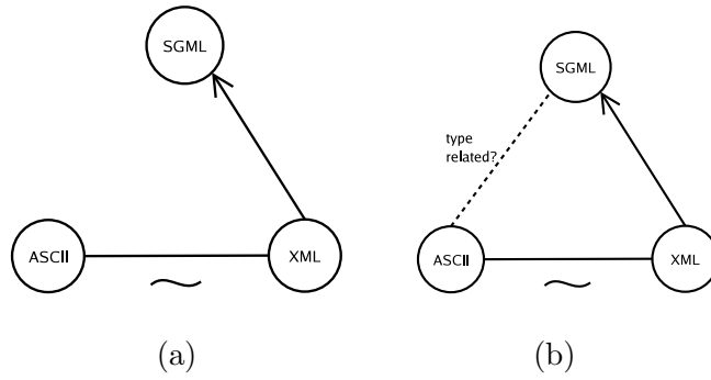
Figure 6. Illustrating Axiom 13
