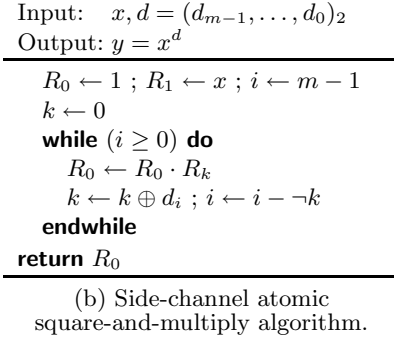
Fig. 2. Protected square-and-multiply algorithm.
