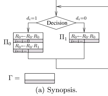
Fig. 2. Protected square-and-multiply algorithm.
