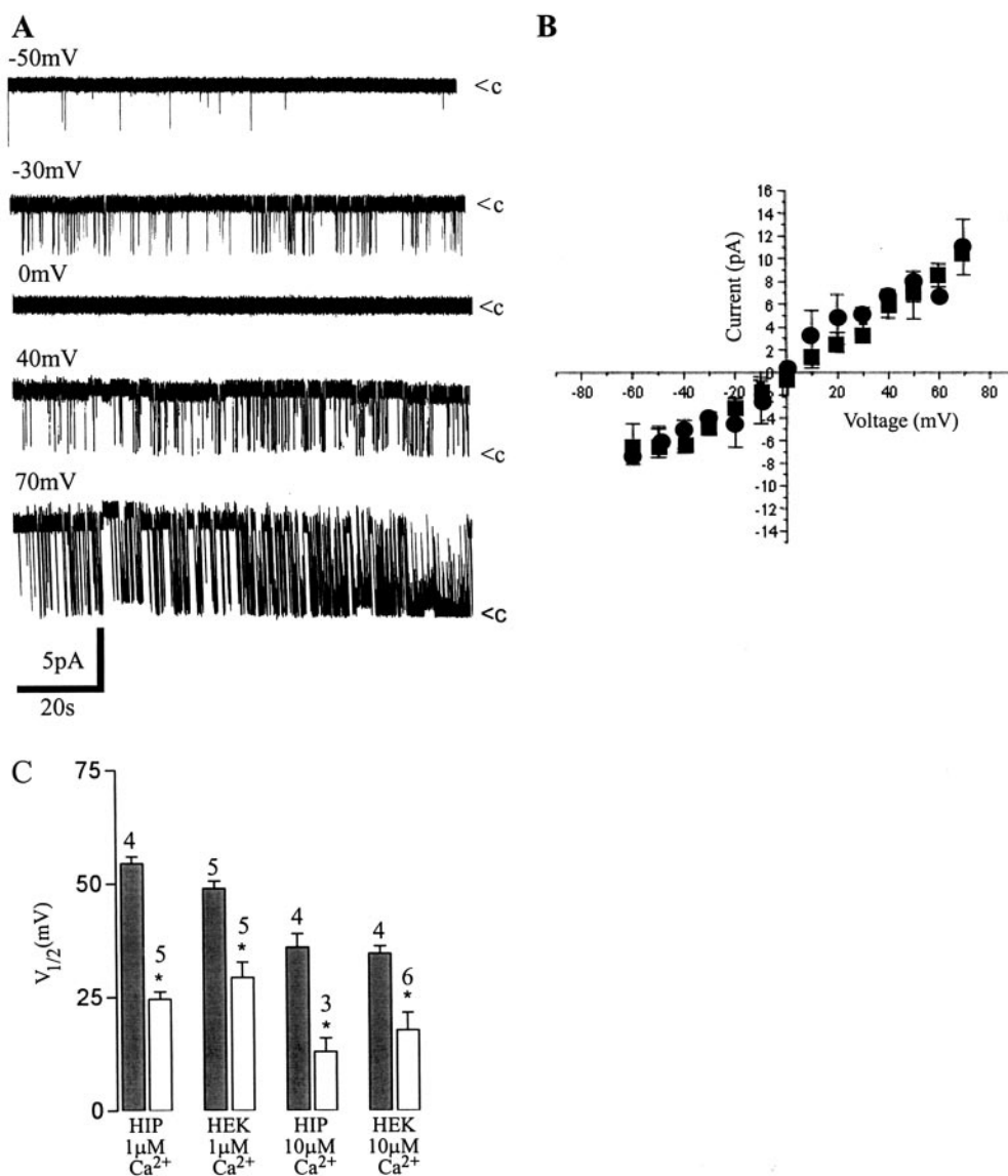
Fig. 4. Characteristics of BK channels after insulin activation. A, sample traces of inside-out recordings from a HEK293 cell obtained in symmetrical 140 mM KCl conditions and in the presence of 1 \mu M Ca^{2+} , after BK channel activation by insulin. Note that in this cell, a small conductance channel is evident at +40 and +70 mV. B, pooled current-voltage relationship of the channel obtained under control conditions (●) or after insulin stimulation (■; obtained 12 to 14 min after activation by insulin) in 1 \mu M Ca^{2+} . C, pooled data illustrating the mean V_{1/2} values obtained in the presence of 1 \mu M or 10 \mu M Ca^{2+} , in cells under control conditions (filled bars), and in distinct cells after exposure to 10 nM insulin (open bars) in both hippocampal neurons (HIP) and HEK293 cells (HEK). The numbers above the histograms represent the n values, and * represents P < 0.05 (Student's t test) for insulin-treated cells compared with control (no insulin treatment) cells under similar conditions.
