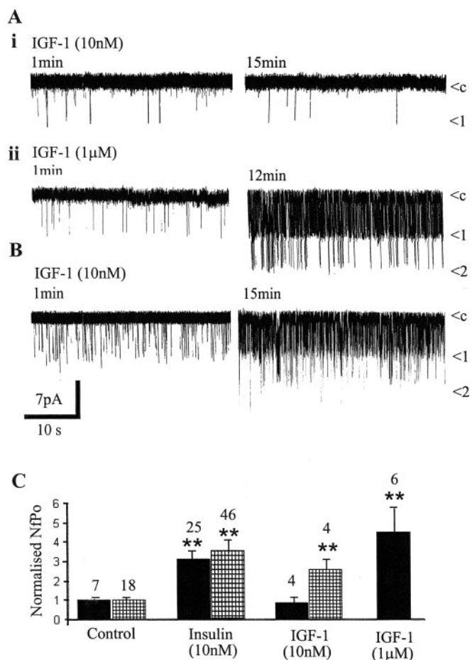
Fig. 3. Insulin and IGF-1 effects on native and recombinant BK channels. A, sample cell-attached recordings from hippocampal neurons with +20 \text{ mV} applied to the recording pipette. Pipette application of IGF-1 ( 10 \text{ nM} ) to hippocampal neurons had no effect on BK channels (Ai). In contrast, IGF-1 ( 1 \mu\text{M} ) evoked an increase in BK channel activity that was maintained in the presence of IGF-1 (Aii). B, Sample cell-attached recordings obtained from HEK293 cells at +10 \text{ mV} applied potential. In these cells, pipette application of IGF-1 ( 10 \text{ nM} ) mimicked insulin action such that an increase in BK channel activity was observed. C, pooled data obtained after 15 min of exposure to insulin or IGF-1, showing the normalized effects of insulin, IGF-1 ( 10 \text{ nM} ), and IGF-1 ( 1 \mu\text{M} ) on channel activity [normalized to the NfP_o values obtained at 2 to 4 min in the same cell in either hippocampal neurons (filled bars) or HEK293 cells (hatched bars)]. The n values for each experimental condition are shown above each histogram bar, and * and ** represent P < 0.05 and P < 0.01 , respectively (paired t test) compared with the corresponding NfP_o values at the 2- to 4-min time point in the same cell.
