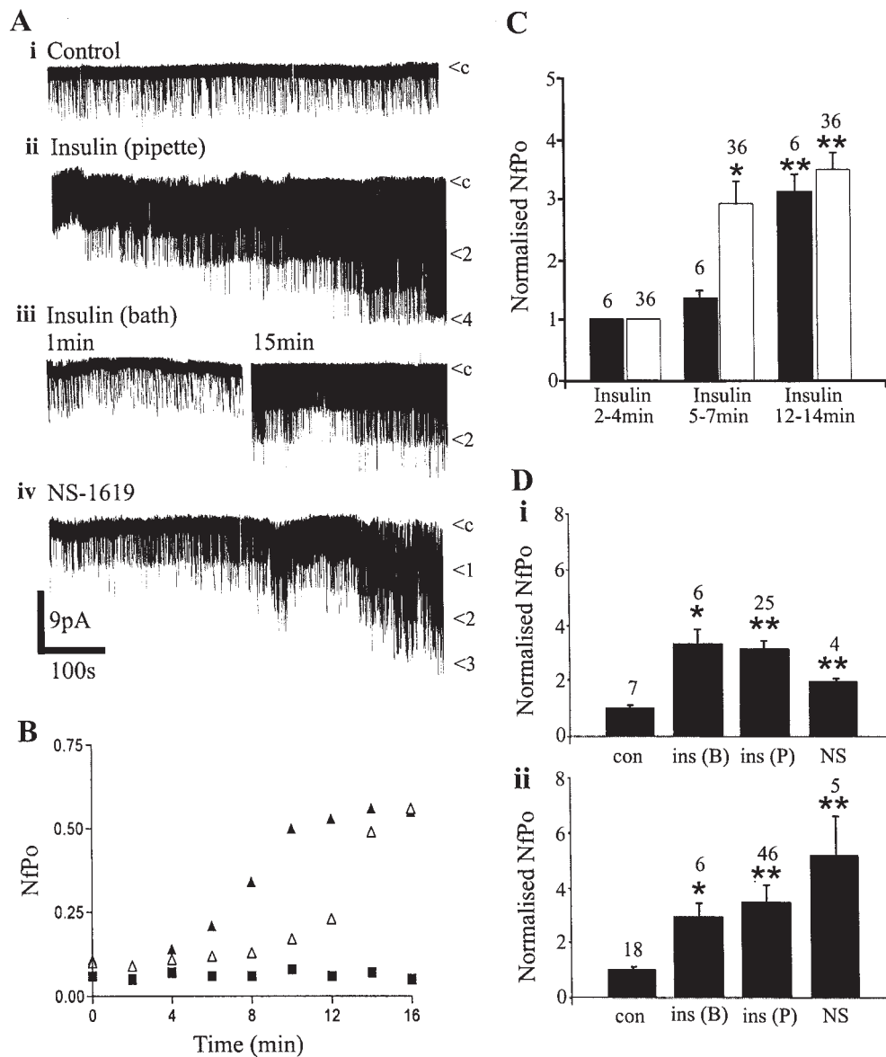
Fig. 2. Insulin activates recombinant ( hSlo ) and native BK channels. A, representative traces of cell-attached recordings from individual HEK293 cells at +10 mV applied to the recording pipette. Ai, under control conditions, there was no change in BK channel activity with time. Aii and Aiii, application of insulin (10 nM) via the patch pipette (P; Aii) or bath (B; Aiii) caused an increase in channel activity that was maintained in the presence of insulin. Aiv, pipette application of the BK channel activator, NS-1619 (10 \mu M), also readily increased the activity of BK channels. B, Plot of the corresponding mean channel activity ( NfP_o ) versus time relations obtained from the experiments illustrated in A (i–iii). Pipette application of insulin (▲) activated BK channels faster than bath application did (△). Control recordings (■) displayed no change in channel activity with time. C, plot of pooled data from HEK293 cells illustrating the pooled normalized NfP_o values obtained 2 to 4 min after the start of recording, and 5 to 7 min and 12 to 14 min after insulin addition, for bath application (filled bars) compared with pipette addition (open bars). Asterisks represent P < 0.05 (one-way ANOVA, repeated measures) relative to the control NfP_o values obtained 2 to 4 min after the initiation of recordings. D, plots of the pooled data obtained 12 to 14 min after insulin addition, showing the relative effects of insulin [bath (B; 50 nM) or pipette (P; 10 nM) application] and NS-1619 (NS; 1 \mu M) on BK channel activity in hippocampal neurons (Di) and HEK293 cells (Dii). All values represent data normalized to a control period, 2 to 4 min after obtaining the cell-attached recording configuration. The n values for each experimental condition are shown above each histogram bar, and * and ** represent P < 0.05 and P < 0.01 compared (paired t test) to the 2- to 4-min time point in the same cell.
