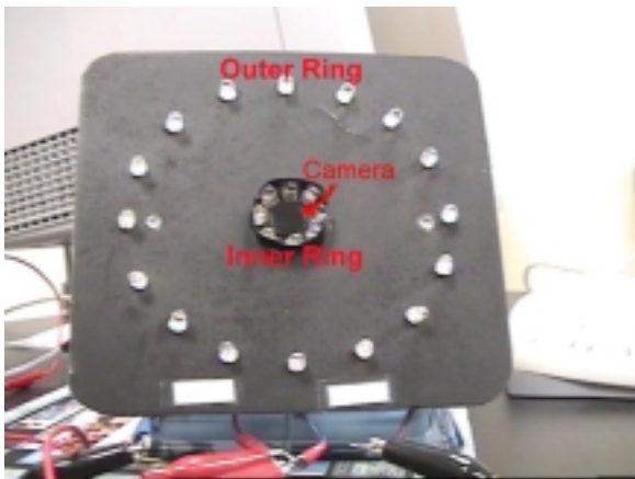
Figure 2: Hardware setup: the camera with active IR illuminations
