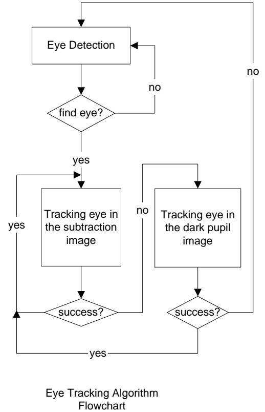
Figure 11: The Eye tracking algorithm flowchart
