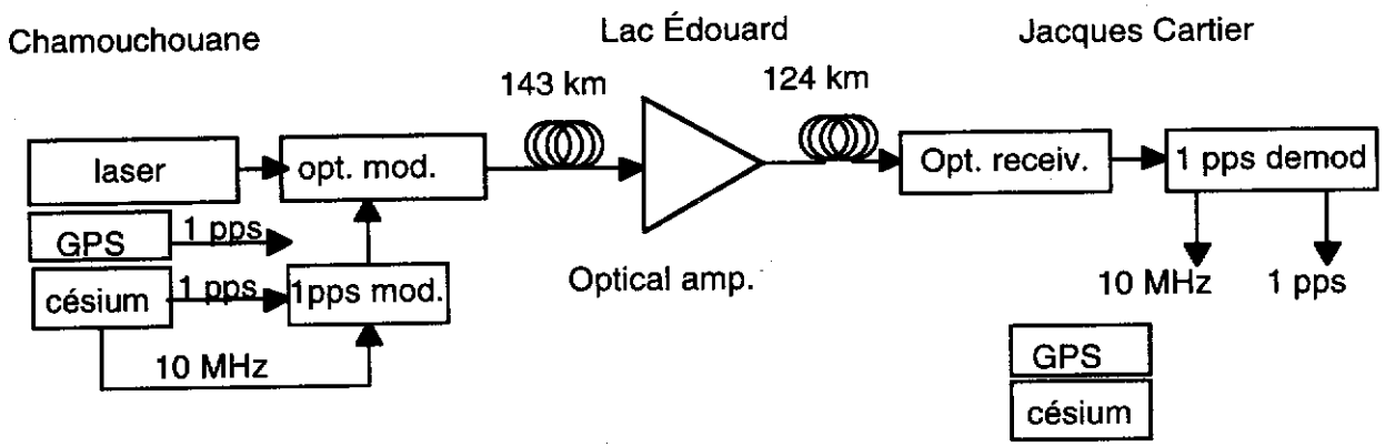
Figure 3. Measurement setup
