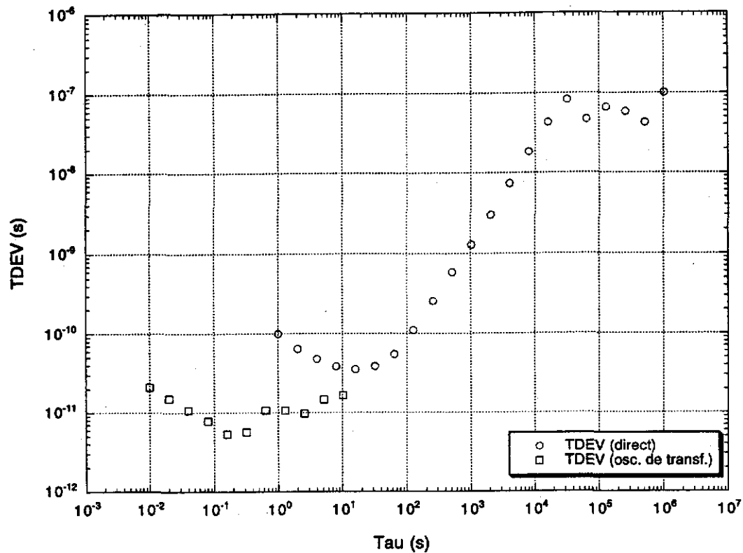
Figure 7. TDEV
