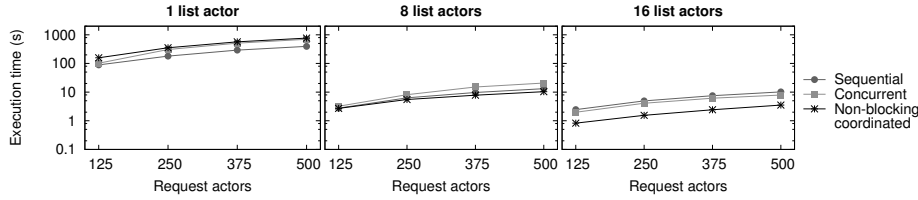
Fig. 7. Execution time for sequential, concurrent, and non-blocking message processing using 1, 8, and 16 list actors on a write-dominated workload.
