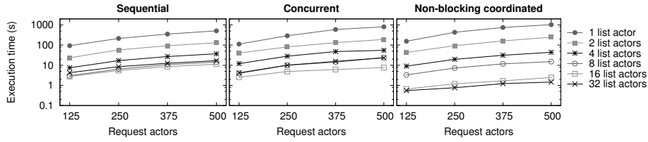
Fig. 6. Execution time for sequential, concurrent, and non-blocking message processing on a write-dominated workload.
