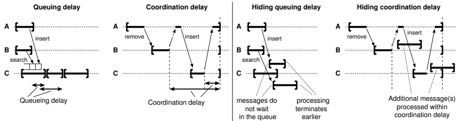
Fig. 1. Sequential (left), concurrent and non-blocking coordinated processing (right) and their effect on execution time.
