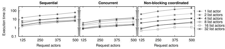
Fig. 4. Execution time for sequential, concurrent, and non-blocking message processing on a read-dominated workload.
