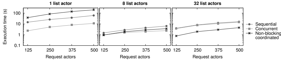
Fig. 5. Execution time for sequential, concurrent, and non-blocking message processing using 1, 8, and 32 list actors on a read-dominated workload.
