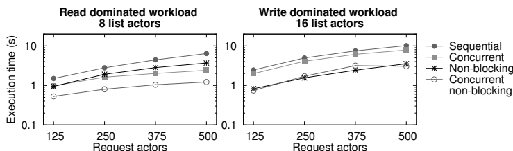
Fig. 8. Execution time for sequential, concurrent, non-blocking, and combined message processing.
