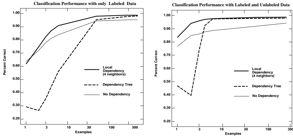
Figure 3: Performance of the three models. X Axis: Amount of labeled training data used. Y Axis: Percent correct on an independent test set. In the left graph, only labeled data was used. In the right graph, unlabeled and labeled data was used (the total number of examples were 500, with varying amounts of labeled data).
