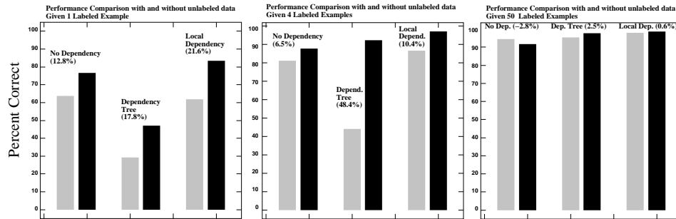
Figure 4: Improvement for each model by using unlabeled data to augment the labeled data. Left: with only 1 labeled example, Middle: 4 labeled, Right: 50 labeled. The bars in light gray represent the performance with only labeled data, the dark bars indicate the performance with the unlabeled data. The number in parentheses indicates the absolute (in contrast to relative) percentage change in classification performance with the use of unlabeled data.
