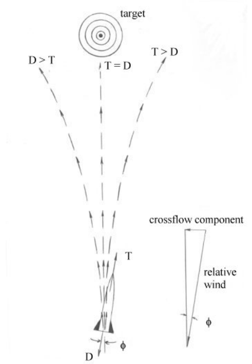
Figure 14. Effects of Crosswind on Drift [see ref. 8]
