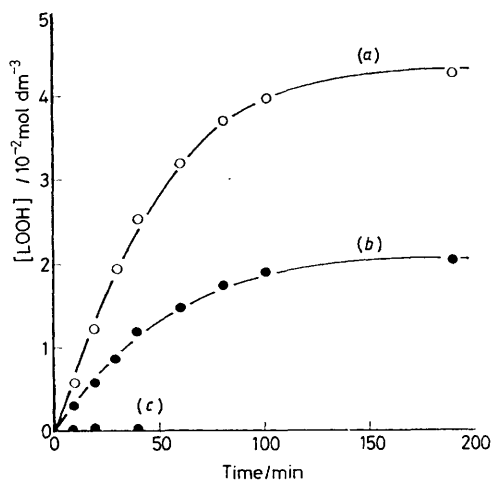
Figure 1. The concentrations of (a) total hydroperoxides and (b) conjugated diene hydroperoxides formed in the FI-sensitized photo-oxidation of linoleic acid ( 0.10 \text{ mol dm}^{-3} ) in the presence of FI ( 9.5 \times 10^{-4} \text{ mol dm}^{-3} ), in an oxygen-saturated MeCN solution under irradiation of light \lambda > 360 \text{ nm} , plotted against the irradiation time, and (c) the inhibitory effect of \text{HClO}_4 ( 1.2 \times 10^{-2} \text{ mol dm}^{-3} ) on the photo-oxidation.
