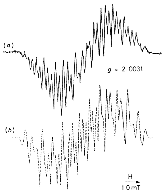
Figure 5. (a) E.s.r. spectrum of \text{FIH}_2^{++} formed in the photo-reduction of \text{FIH}^+ by linoleic acid in deaerated MeCN. (b) The dotted line shows the corresponding computer simulation spectrum using the e.s.r. parameters listed above.
