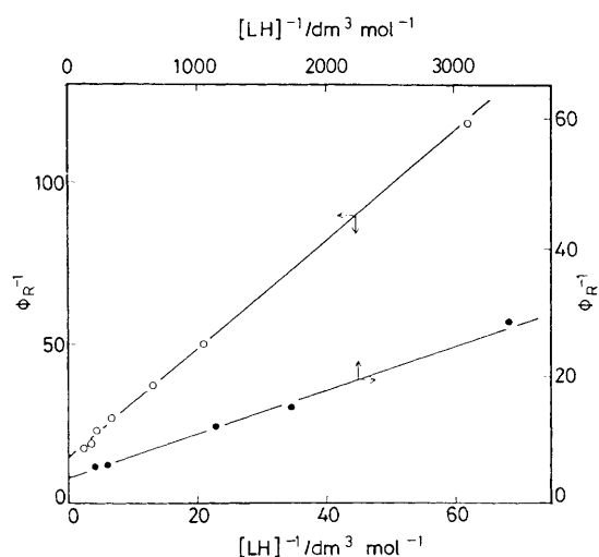
Figure 6. Plots of \phi_R^{-1} vs. [\text{LH}]^{-1} for the photo-reduction of \text{FIH}^+ ( 1.5 \times 10^{-4} \text{ mol dm}^{-3} ) by linoleic acid (LH) in the absence ( \circ ) and presence ( \bullet ) of \text{HClO}_4 ( 1.2 \times 10^{-2} \text{ mol dm}^{-3} ) in deaerated MeCN under irradiation of light of \lambda 442 and 390 nm, respectively.
