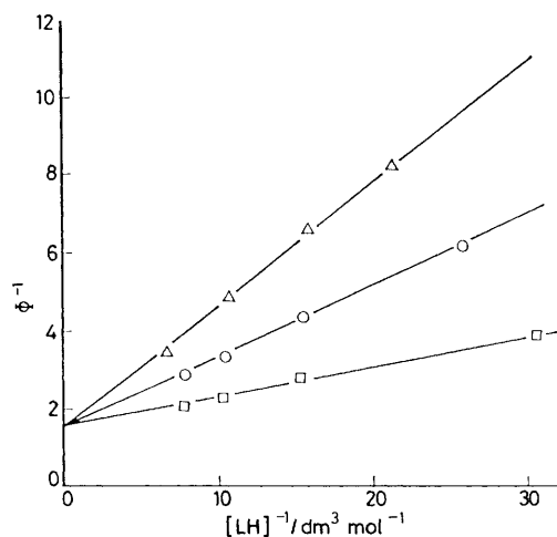
Figure 3. Plots of \phi^{-1} vs. [\text{LH}]^{-1} for the Fl-sensitized photo-oxidation of oleic acid ( \Delta ), linoleic acid ( \circ ), and linolenic acid ( \square ) in the presence of Fl ( 1.5 \times 10^{-4} \text{ mol dm}^{-3} ) in an oxygen-saturated MeCN solution under irradiation of light of \lambda 442 nm.
