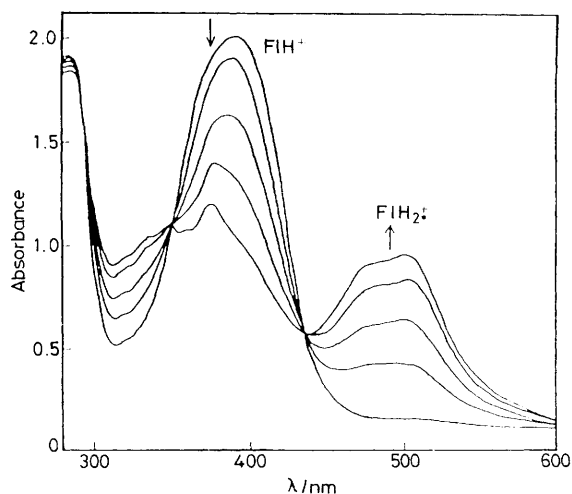
Figure 4. Electronic absorption spectra observed in the photochemical reaction of \text{FIH}^+ ( 1.2 \times 10^{-4} \text{ mol dm}^{-3} ) with linoleic acid ( 8.1 \times 10^{-3} \text{ mol dm}^{-3} ) in the presence of \text{HClO}_4 ( 1.2 \times 10^{-2} \text{ mol dm}^{-3} ) in deaerated MeCN. The spectra were recorded after each 30 s irradiation of light of \lambda 390 nm.
