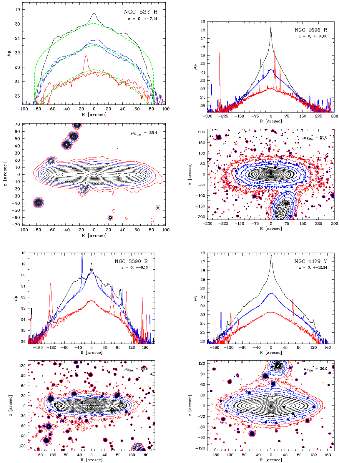
Figure B1. Radial surface brightness profiles and isophote maps for NGC 522 R-band, NGC 1596 R-band, NGC 3390 R-band, and NGC 4179 V-band (from top left to bottom right).
