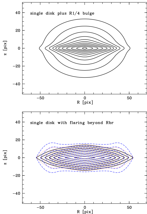
Figure 9. Upper panel: Contour map of a radially broken exponential, vertically exponential thin disk superimposed with a standard de Vaucouleurs R^{1/4} bulge. Lower panel: Three combination of a the same thin disk and a thick disk, where the thick disk scaleheight grows (flares) between the break radius ( R_{\text{br}} ) and three times R_{\text{br}} with an increasing factor ( solid, dashed, dotted lines ).
