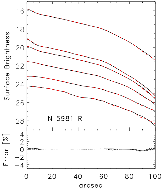
Figure 2. Test of deprojection method for NGC 5981.
