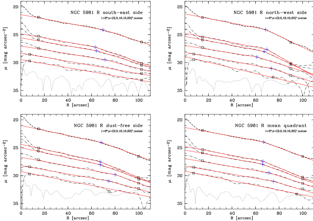
Figure 4. Influence of asymmetries: Averaging quadrants
