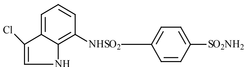
Figure 5. Chemical structure of E7070; a novel synthesized sulfonamide with anticancer effects.
