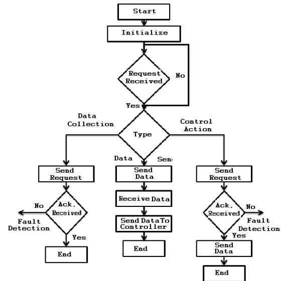
Figure 7: Coordinator Agent Software Flow.
