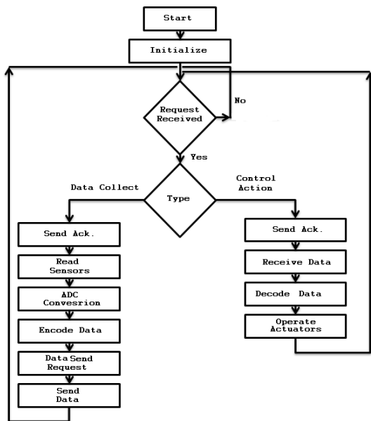
Figure 6: Local Station Data Flow.
