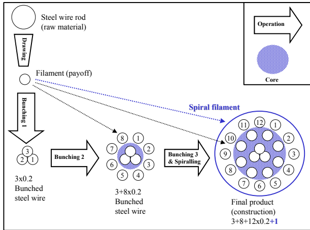
Figure 3: Cross-section of 3+8+12x0.2+1 Construction at Successive Bunching Operations
