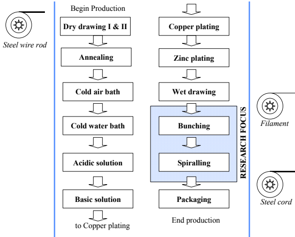
Figure 2: Production Processes in Steel Cord Manufacturing
