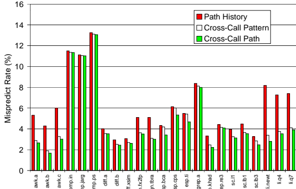
Figure 12. Mispredict rates of scbp using path history (same as the third series in Figure 6) and simulated mispredict rates for cross-call pattern and cross-call path history dividers with static predictors. These results use a history depth of 12 and train and test on the same dataset.
