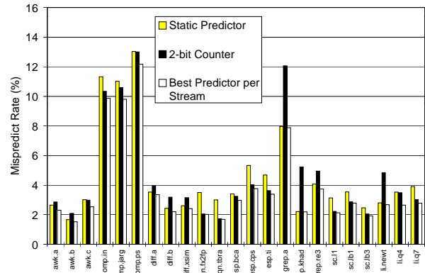
Figure 16. Mispredict rates under an unaliased, cross-call, path divider, comparing assigning all streams to perfectly trained static predictors (“Static Predictor”), all streams to 2-bit counters (“2-bit Counter”), and the best predictor for an entire stream to that stream (“Best Predictor per Stream”).
