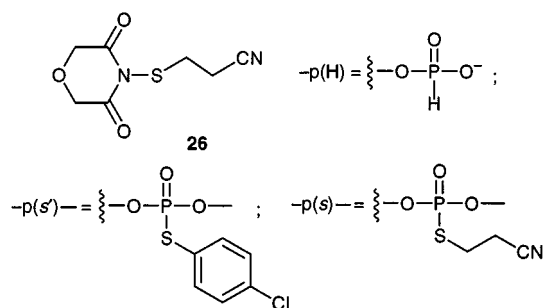
Scheme 6 Reagents and conditions: i, 22 , \text{C}_5\text{H}_5\text{N} , \text{CH}_2\text{Cl}_2 , -40^\circ\text{C} , 10 min; ii, a, 23a , \text{C}_5\text{H}_5\text{N} , \text{CH}_2\text{Cl}_2 , -40^\circ\text{C} , 15 min, b, \text{C}_5\text{H}_5\text{N} -water (1:1 v/v); iii, 4\text{ mol dm}^{-3} \text{HCl} /1,4-dioxane, \text{CH}_2\text{Cl}_2 , -50^\circ\text{C} , 5 min; iv, 26 , \text{C}_5\text{H}_5\text{N} , \text{CH}_2\text{Cl}_2 , -40^\circ\text{C} , 10 min.
