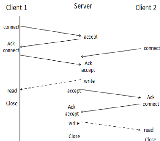
Figure 2:-Iterative server Model working
