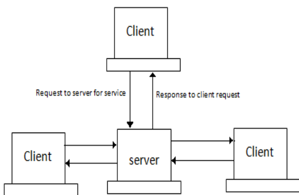
Figure 1: - Client-Server Model
