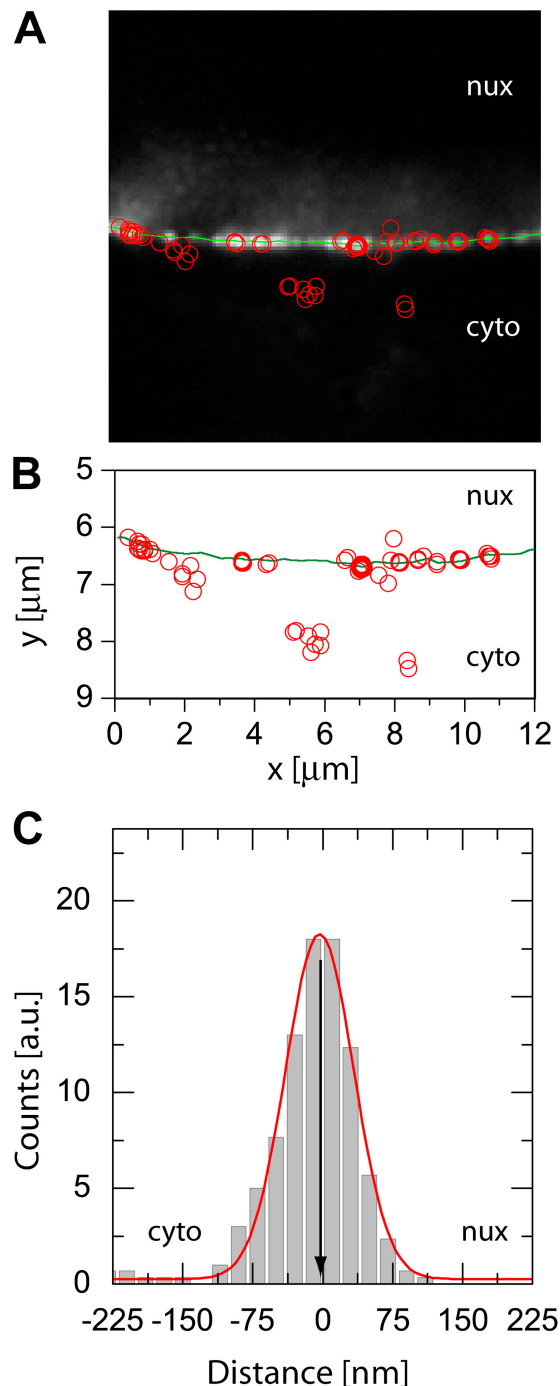
Figure 3. Single \text{kap}\beta 1 \Delta N44 molecules at the NE. For a single cell, all fitted positions (open red circles) were overlaid with the image of the NE. The estimate of the NE position was indicated by a green line in A and B. \text{kap}\beta 1\Delta N44 molecules were preferentially observed at the GFP-labeled NPCs, while molecules were only very rarely observed within unlabeled regions of the NE. The fitted positions of both the NE and the single molecules were plotted to scale in B. The individual distances of the \text{kap}\beta 1\Delta N44 molecules from the NE were calculated as the shortest distances between the fitted position of the single molecule and the nearest point on the fit through the NPC signals marking the NE. The resulting distance distribution of \text{kap}\beta 1\Delta N44 molecules to the NE is shown in C. The position of the NE was defined as zero. Then, negative values described a single molecule position at the cytoplasmic face of the NPC, positive values at the nucleoplasmic face. A fit to a Gaussian yielded a maximum position of the distribution at -3 \pm 1 nm with a width (FWHM) of 80 \pm 2 nm.
