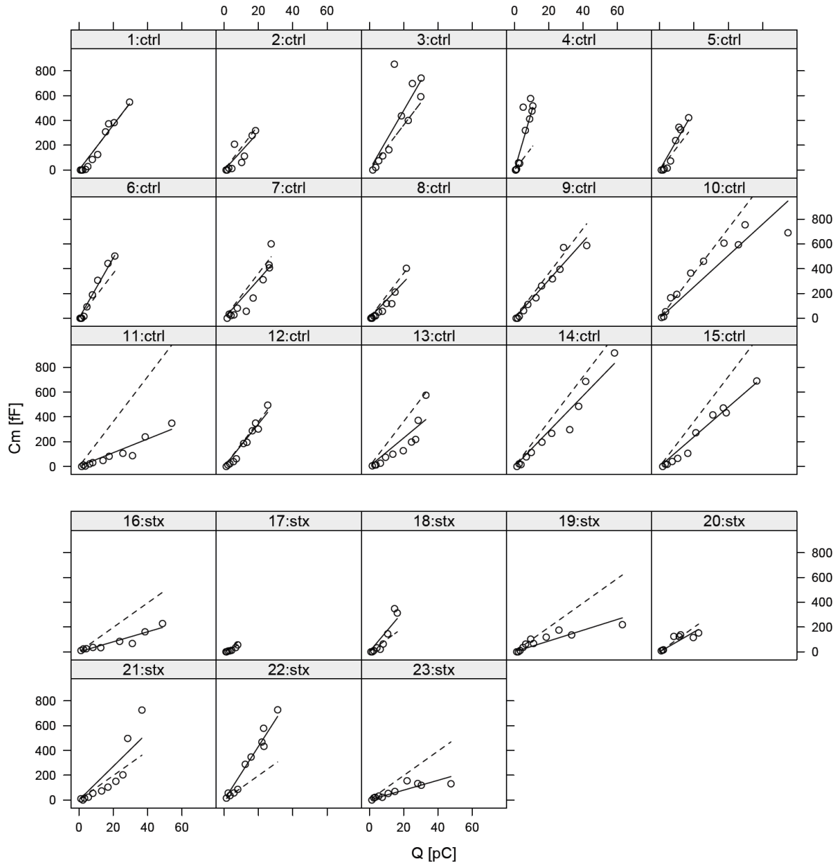
Suppl Fig. 2. Mixed-effects statistical model to estimate the Ca^{2+} -sensitivity of exocytosis. The graphs describe the results from individual experiments under control conditions (ctrl) or in the presence of anti-syntaxin 1A (stx) from the experiments presented in Fig. 4. Data for the individual experiments are presented as the increase in membrane capacitance ( C_m ) as a function of the Ca^{2+} -charge ( Q ). The fixed effect of Ca^{2+} on exocytosis, which quantifies the Ca^{2+} -sensitivity within each group, is indicated by the dotted line. The fits to data from individual experiments are indicated by the black, full curves. The random effect representing cell-to-cell variation accounts for the difference between cell (full) and group (dashed) fits.
