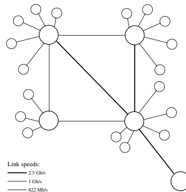
Fig. 10. simulated GARR network topology
