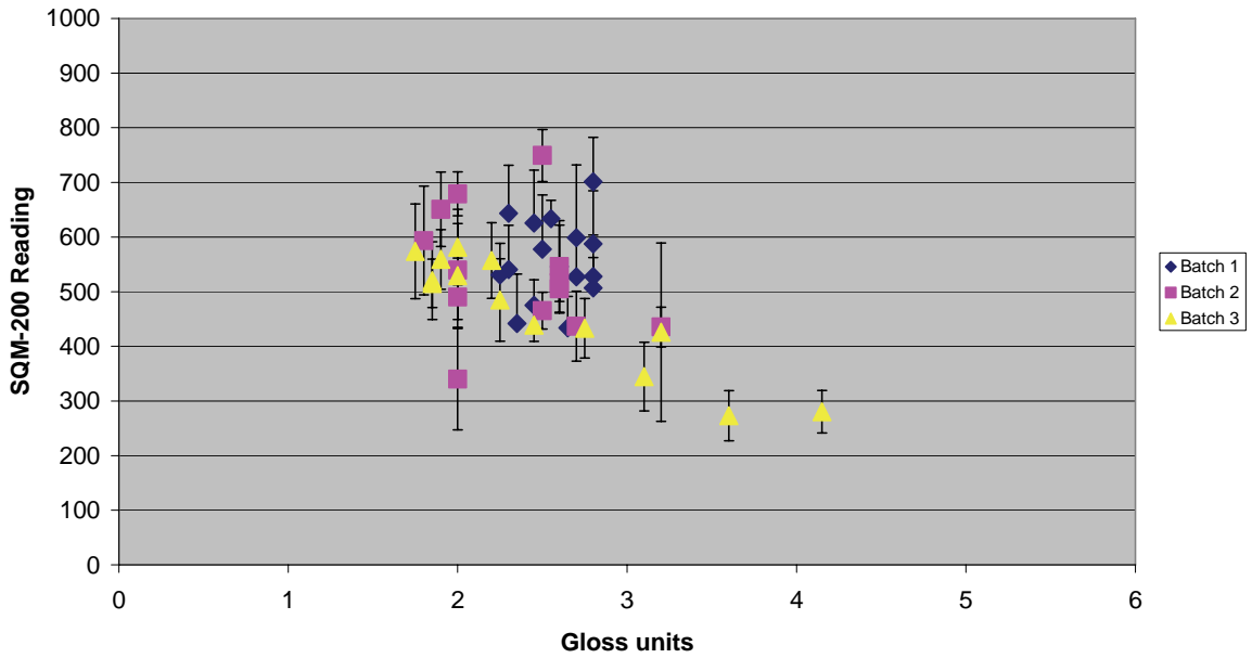
Figure 14 SQM-200 measurements taken on grit-blasted clad Al2024-T3 aluminium plates used for wedge test manufacture plotted as a function of gloss units.
