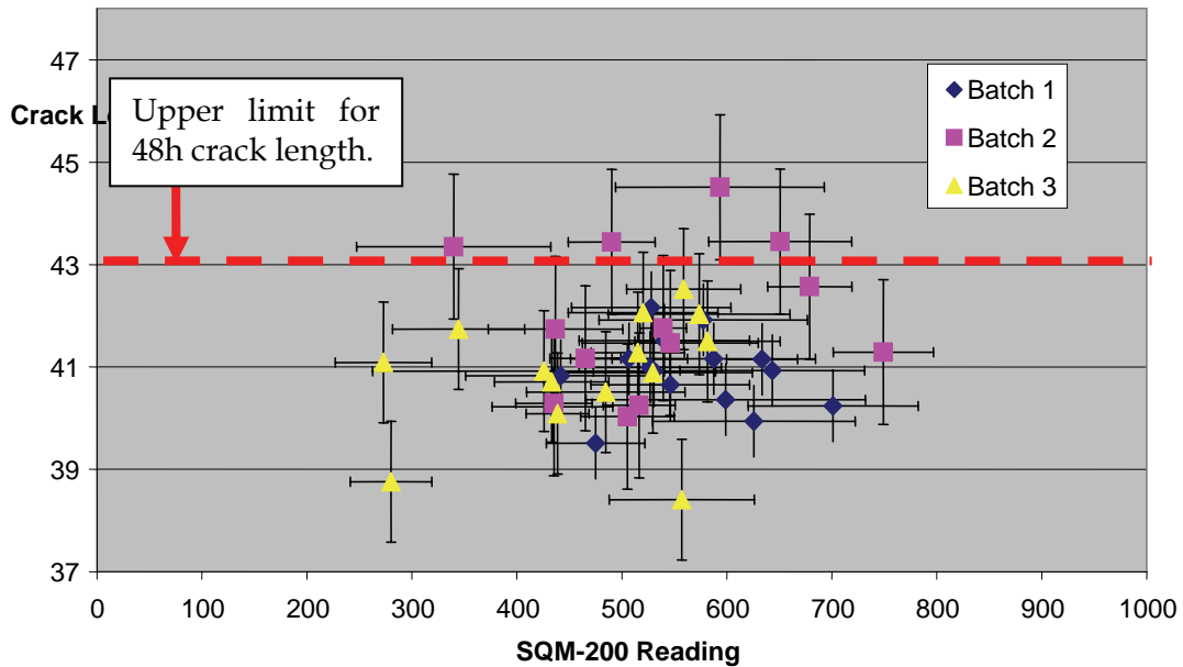
Figure 15 Crack length measured after 48 hours humid exposure for wedge test samples where the grit-blast surface was measured with the SQM-200 prior to bonding.
