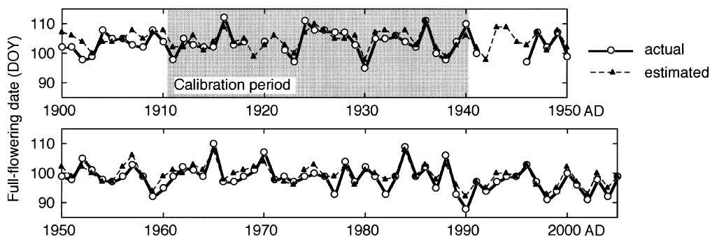
Figure 3. Actual and estimated full-flowering dates of the cherry tree, P. jamasakura . Dates were estimated by using suitable values for the variables D and E_a in the DTS model.
