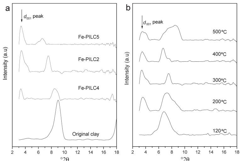
Figure 3. XRD patterns of (a) Fe-PILCs prepared using different OH/Fe molar ratios and calcined at 300^\circ\text{C} and, (b) Fe-PILC2 calcined at different temperatures.
