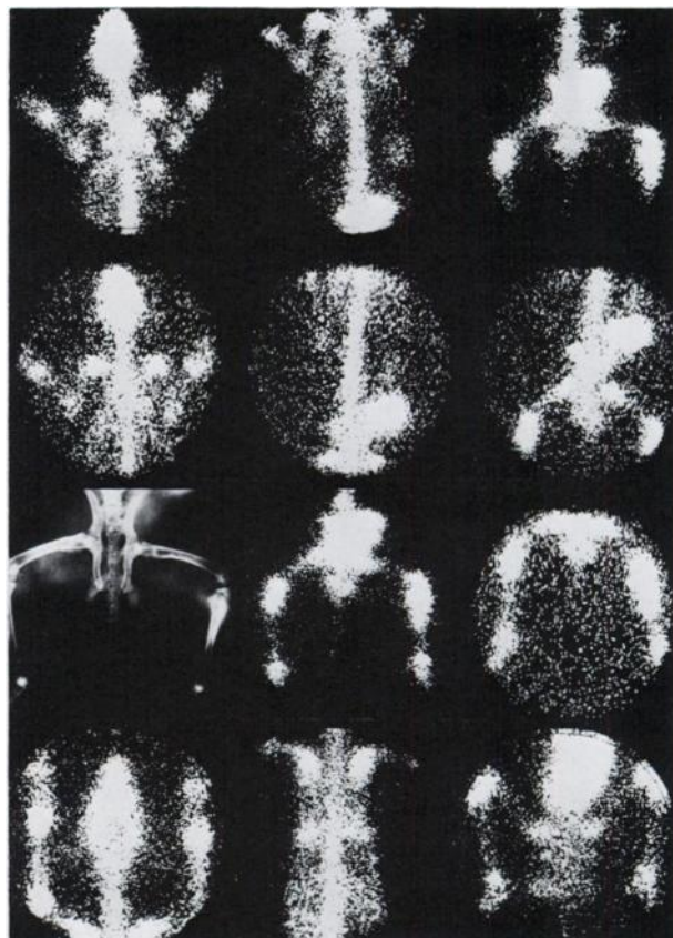
FIG. 1. Camera images after 3-mCi ^{157}\text{Dy} -HEDTA. Rabbit at 4 hr (top row) and 24 hr (second row). Radiograph, 4- and 24-hr images of fibial fracture site shown in third row. Images obtained in normal dog at 6 hr (bottom row).
