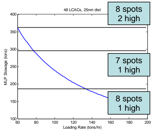
Figure 34. Case #52 / 48 LCACs / 25 nm
