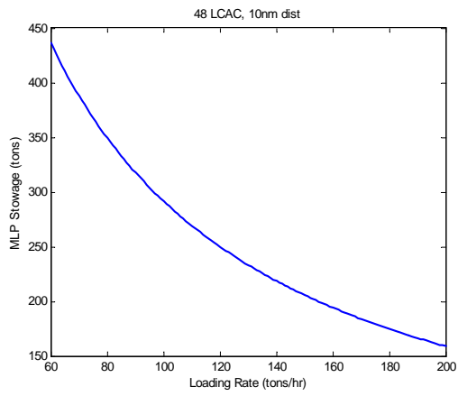
Figure 28. Case #20 / 48 LCACs/ 10 nm
