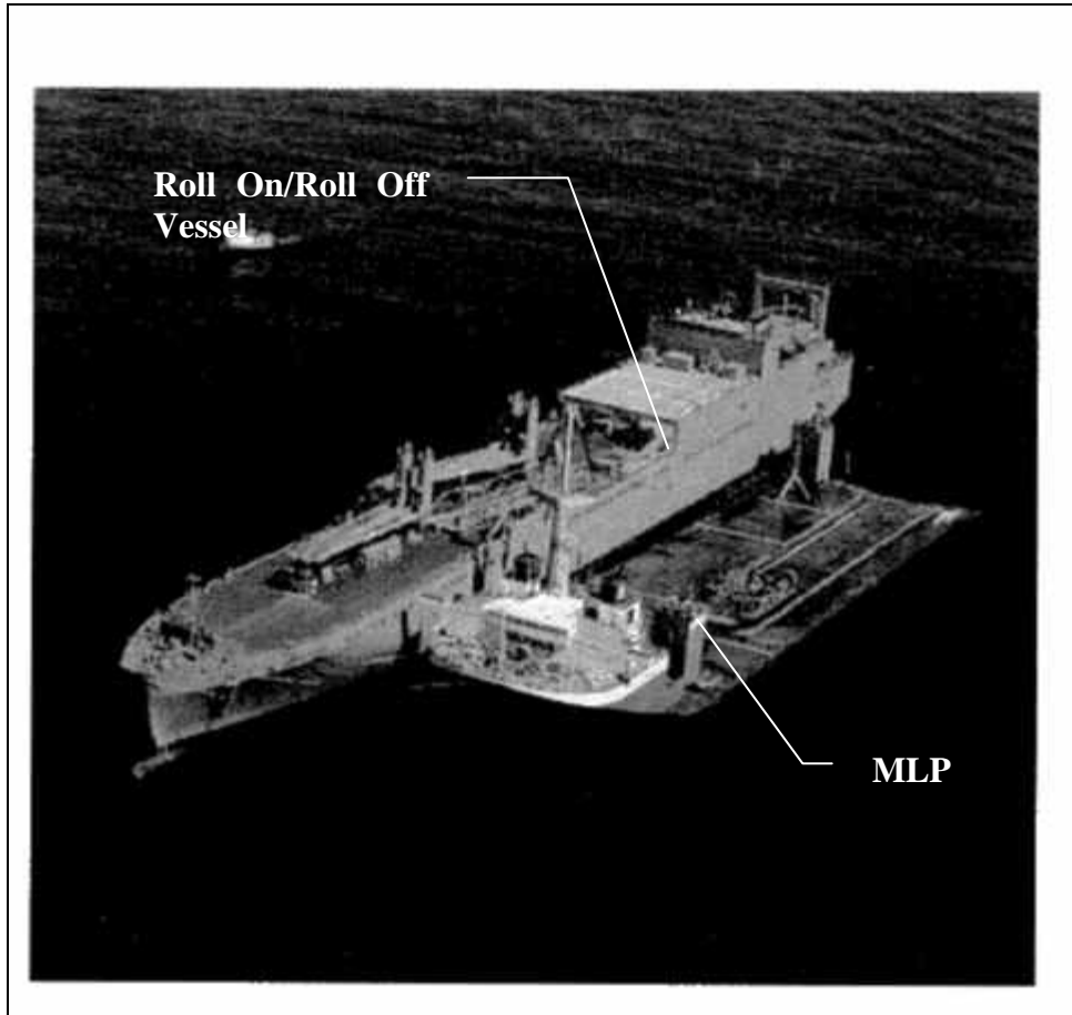
Figure 10. MIGHTY SERVANT 1 and WATKINS Moored Skin-to-Skin From [12]
