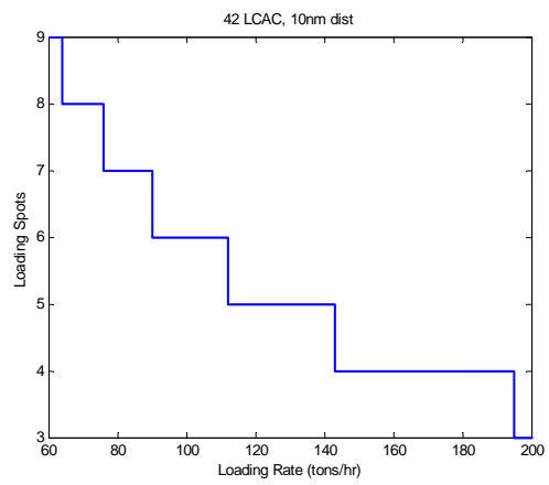
Figure 27. Case #17 / 42 LCACs/ 10 nm
