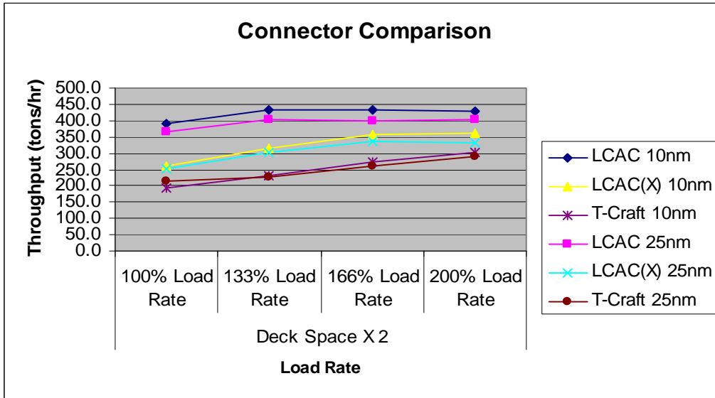
Figure 62. Throughput Rate (tons/hr) Deck Space X 2
