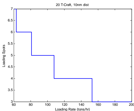
Figure 55. Case #112 / 20 T-Craft / 10 nm
