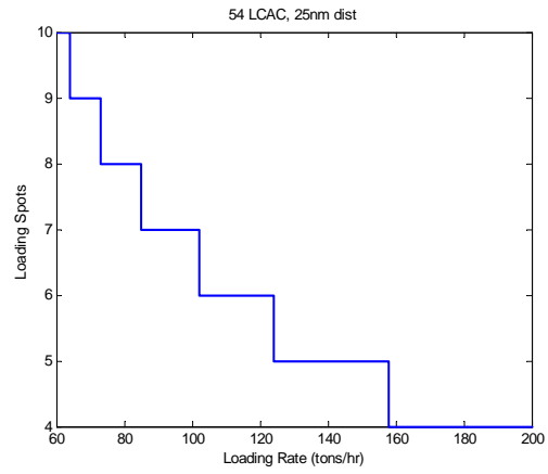
Figure 35. Case #55 / 54 LCACs / 25 nm
