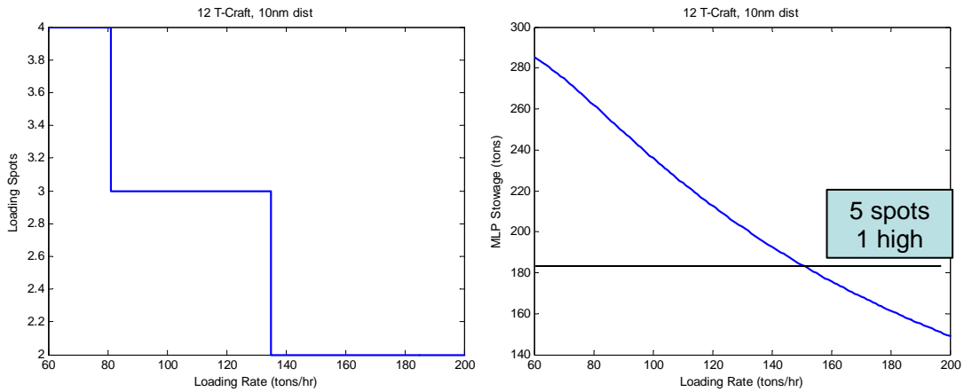
Figure 51. Case #108 / 12 T-Craft / 10 nm
