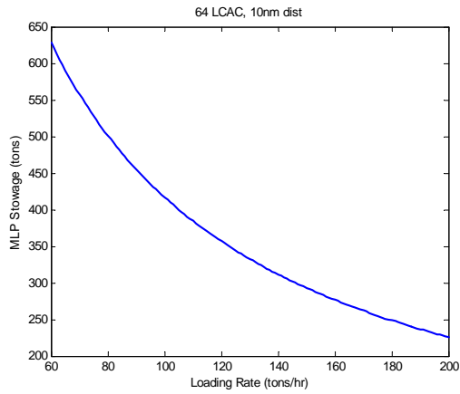
Figure 31. Case #29 / 64 LCACs/ 10 nm
