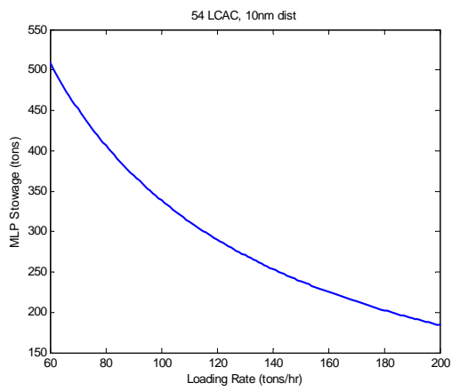
Figure 29. Case #23 / 54 LCACs/ 10 nm
