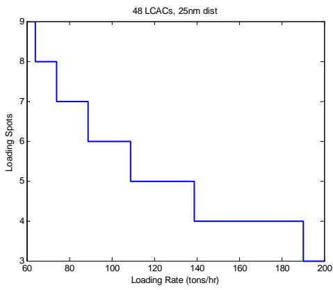
Figure 34. Case #52 / 48 LCACs / 25 nm
