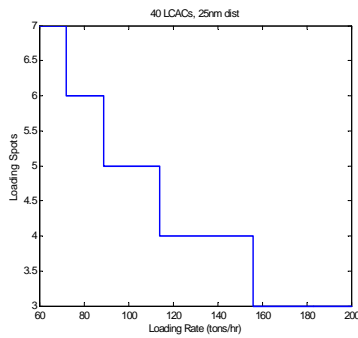
Figure 32. Case #48 / 40 LCACs / 25 nm
