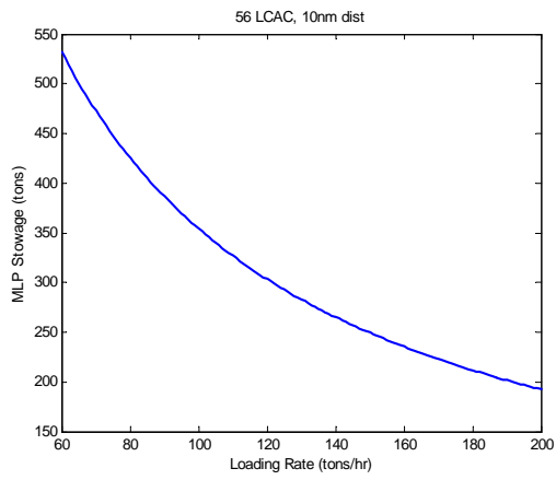
Figure 30. Case #24 / 56 LCACs/ 10 nm
