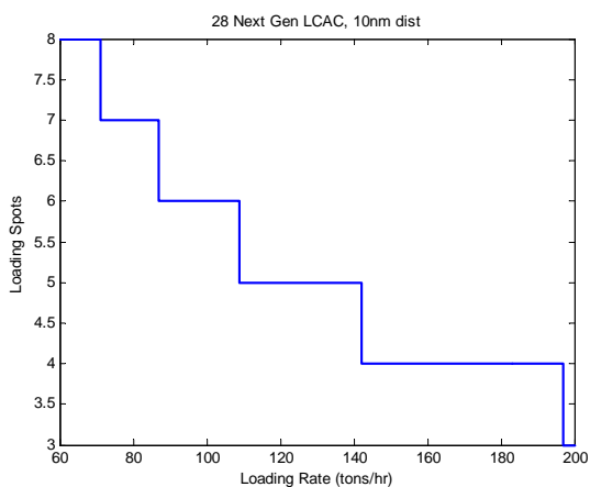
Figure 43. Case #80 / 28 Next Generation LCACs / 10 nm
