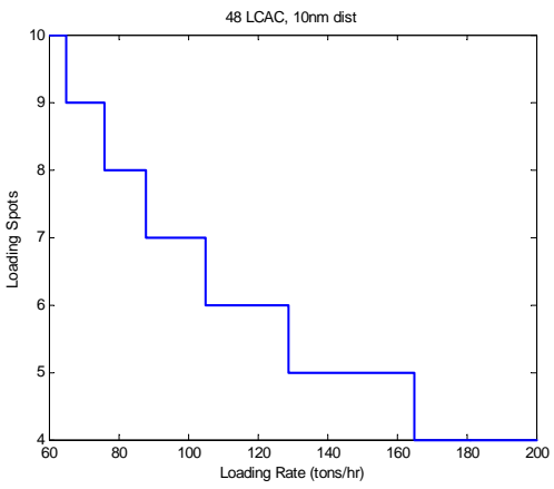
Figure 28. Case #20 / 48 LCACs/ 10 nm
