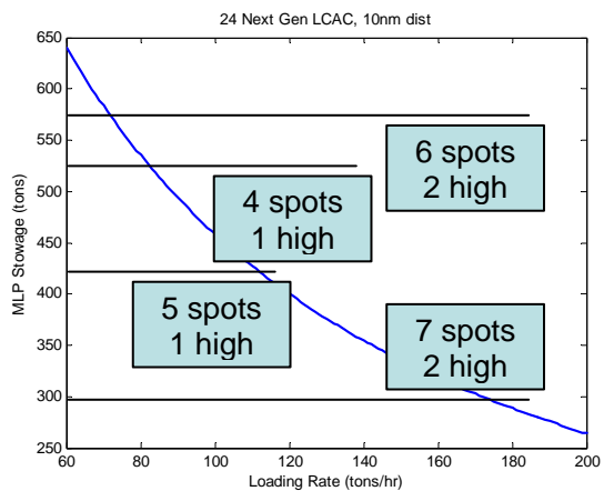
Figure 42. Case #78 / 24 Next Generation LCACs / 10 nm
