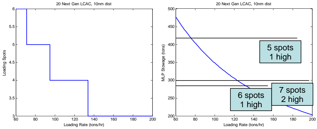
Figure 40. Case #76 / 20 Next Generation LCACs / 10 nm
