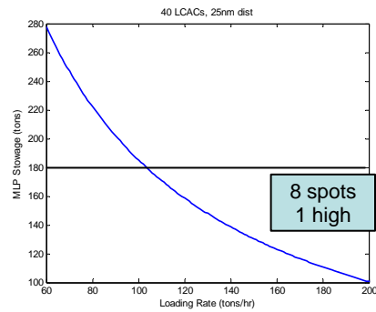
Figure 32. Case #48 / 40 LCACs / 25 nm
