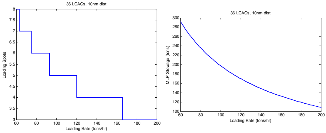
Figure 25. Case #14 / 36 LCACs / 10 nm
