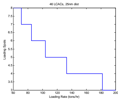
Figure 33. Case #51 / 46 LCACs / 25 nm
