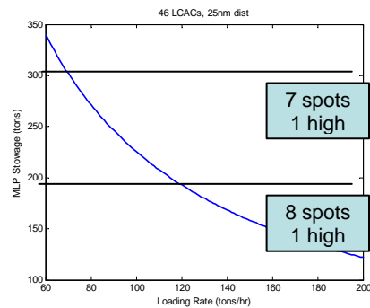
Figure 33. Case #51 / 46 LCACs / 25 nm
