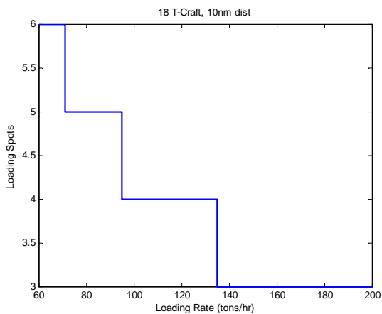
Figure 54. Case #111 / 18 T-Craft / 10 nm
