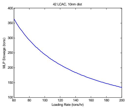
Figure 27. Case #17 / 42 LCACs/ 10 nm
