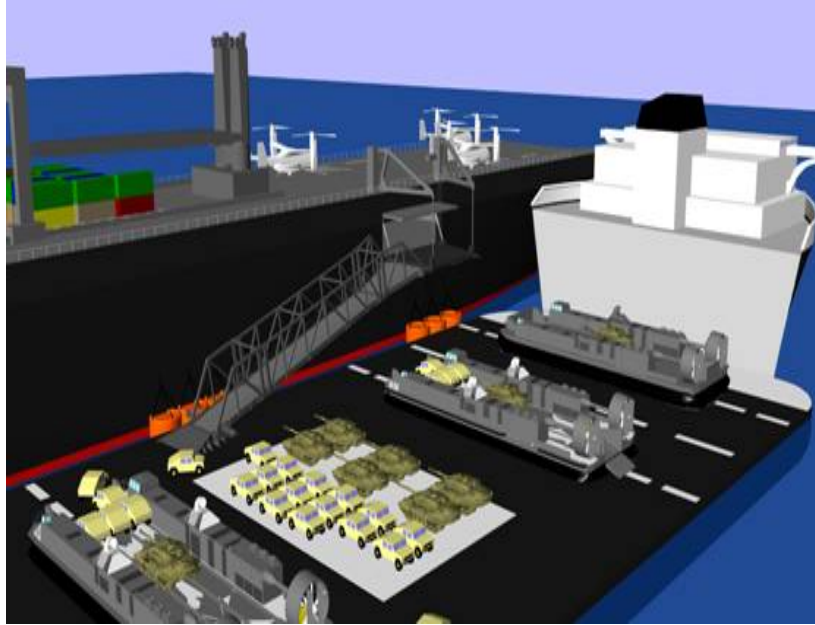
Figure 5. Interface Ramp Technologies From [7]
