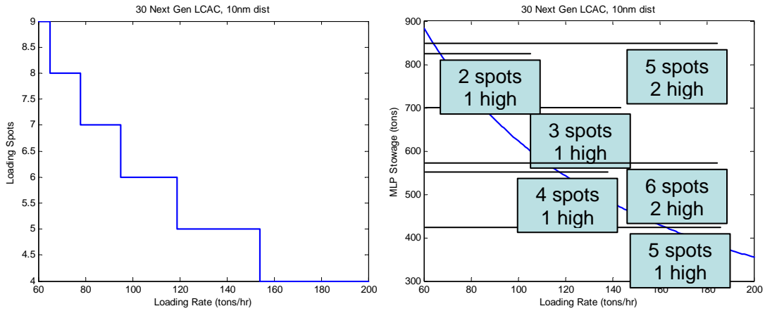
Figure 44. Case #81 / 30 Next Generation LCACs / 10 nm
